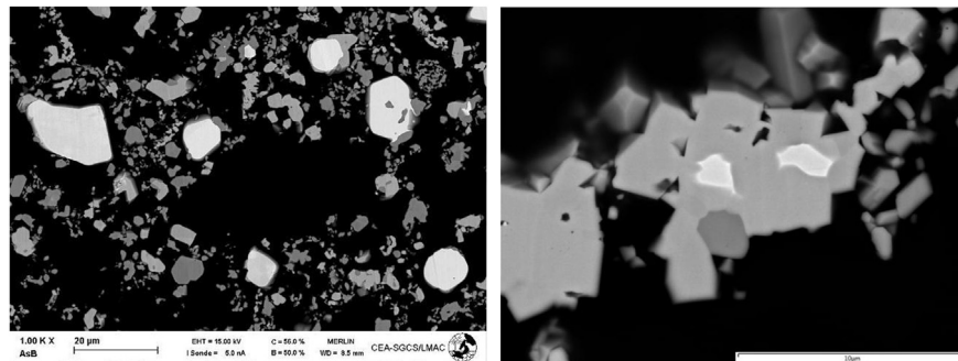
Fig. 6. SEM pictures of sample B. The bright grey phase is \text{Rh}_2\text{O}_3 ; the dark grey phase is the rutile phase (\text{Ru,Rh})\text{O}_2 and the white phase is the metallic solid solution (Rh)-FCC.
