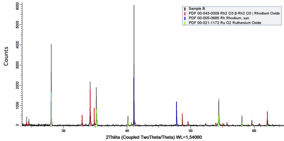
Fig. 5. X-ray powder diffraction diagram of sample B with signal K\alpha_2 subtraction. Indexation with PDF files 2016: 00-043-0009 for \text{Rh}_2\text{O}_3 , 00-005-0685 for (Rh,Ru)-FCC and 00-021-1172 for (\text{Ru,Rh})\text{O}_2 .
