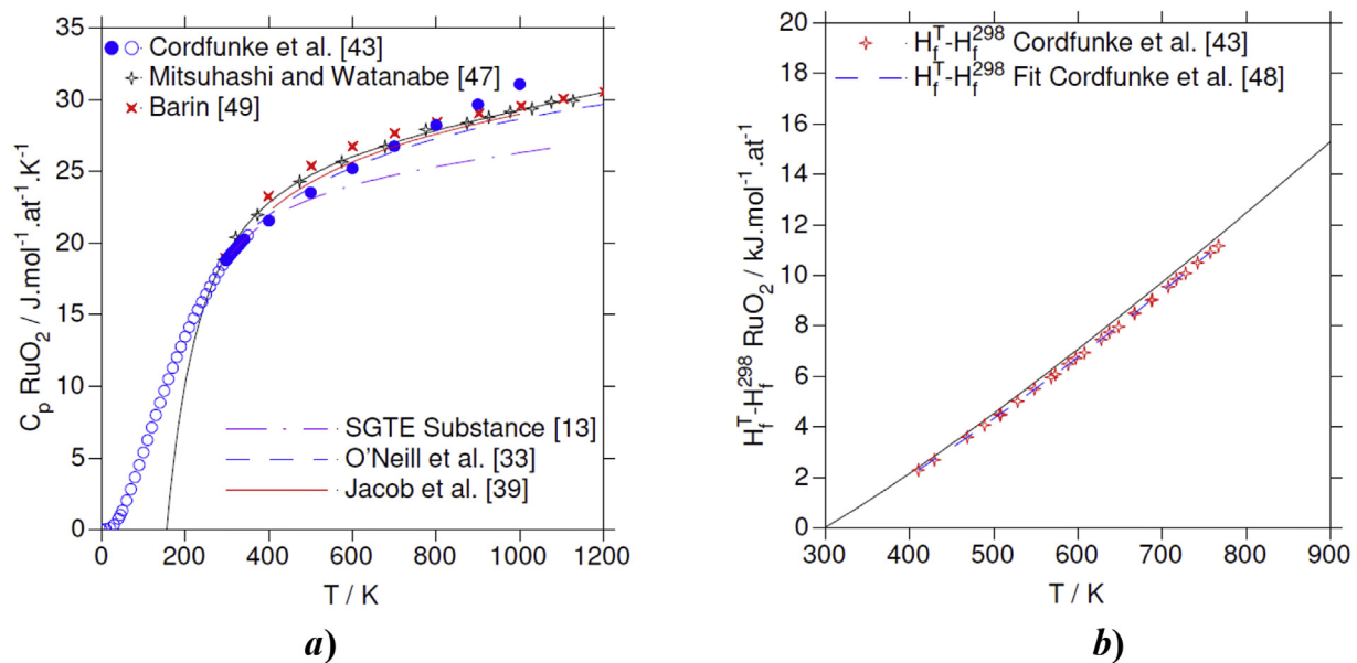
Fig. 4. a) Heat capacity of RuO 2 , comparison with SGTE [13], O'Neill [33], Jacob et al. [39], Cordfunke et al. [43], Mitsuhashi and Watanabe [47] and Barin [49] and b) Enthalpy increment of RuO 2 , comparison with Cordfunke et al. [43,48].
