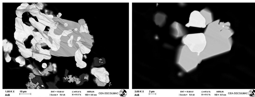
Fig. 7. SEM pictures of sample E. The grey phase is \text{RuO}_2 ; there are two shades in the white phase, which are the metallic solutions \text{Rh}_{0.7}\text{Ru}_{0.3} and \text{Rh}_{0.6}\text{Ru}_{0.4} .
