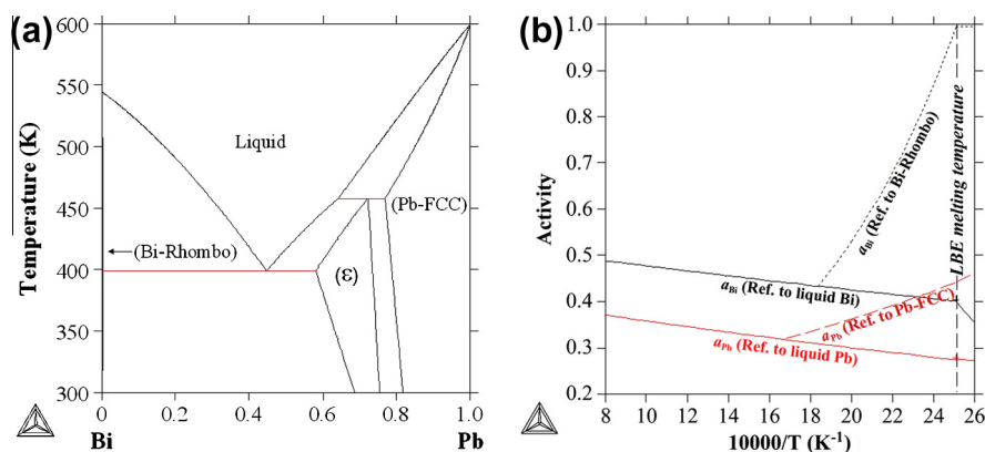
Fig. 1. (a) Bi–Pb phase diagram after Yoon and Lee [3] and (b) Bi and Pb chemical activities calculated at LBE composition as a function of the inverse of temperature: solid lines are referred to pure Bi (black) and Pb (red) liquids, red dash line is referred to Pb–FCC and black dot line is referred to Bi-Rhombohedral. (For interpretation of the references to color in this figure legend, the reader is referred to the web version of this article).
