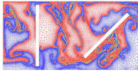
(c) t = \pi .
