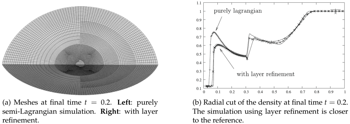
Figure 2.12: Illustration of the effect of the dynamic layer refinement effect on a converging Sod shock tube in 3D.
