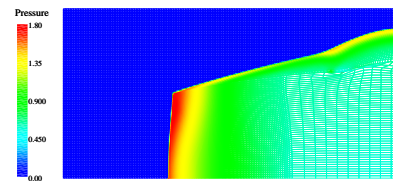
(a) Initial 100 \times 50 mesh.
