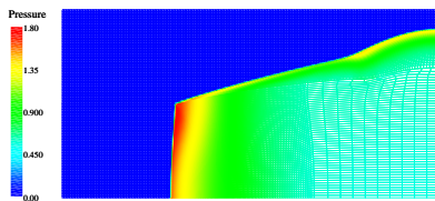
(b) Pressure field — Time t = 0.3 . Mesh 200 \times 100 . Lagrangian simulation with stabilization.
