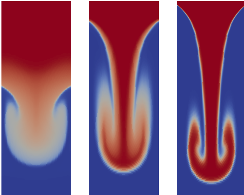
Figure 2.11: 80 \times 224 mesh. Time t = 0.7 . Mass fraction of fluid \alpha . Influence of the friction parameter. Left: \nu = 100 . Middle: \nu = 1000 . Right: \nu = 10^6 .
