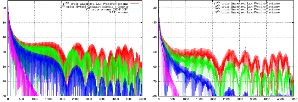
(a) Comparison of various schemes on a fine grid (15 cells per wavelength)
