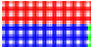
(a) Initial 100 \times 50 mesh.
