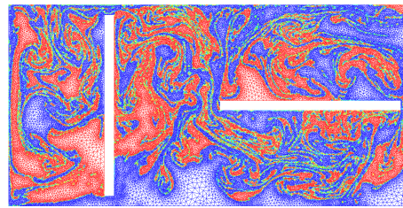
(e) t = 2\pi .
