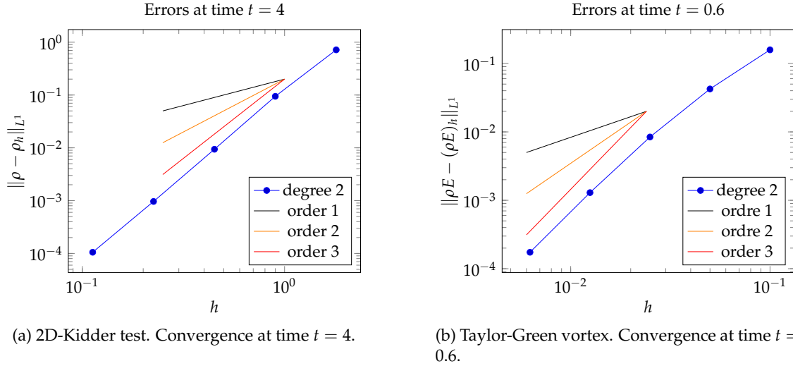
Figure 2.6: Third-order preliminary results obtained with P. Hoch and E. Labourasse. We use a \mathbb{P}^2 -isoparametric discretization to compute \mathbf{u}^* . The loss of coercivity related to this discretization and its treatment are not discussed in this document.
