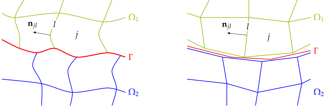
(a) Example of curved meshes which match perfectly the sliding interface.
