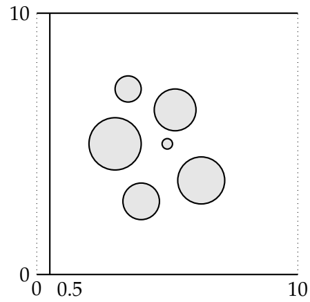
(a) Initial geometry for the shock interaction with cylindrical bubbles.
