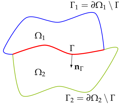
Figure 2.7: The fluids in \Omega_1 and \Omega_2 are sliding on the interface \Gamma .
