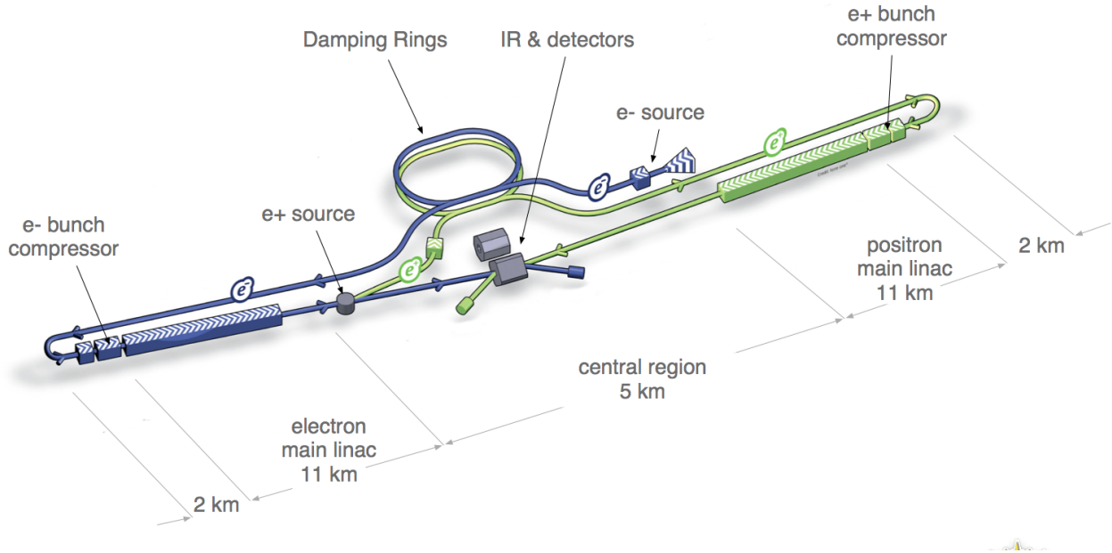
Figure 5.1: (Basic layout of the International Linear Collider.
