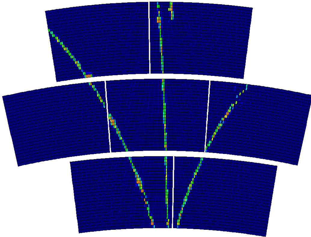
Figure 5.12: Picture of 4 GeV electron beam event recorded by the 7 modules (Run 3050, evt 33).
