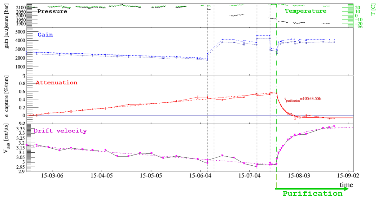
Figure 6.8: Time evolution of the gain, the attenuation an the drift velocity. For the first 5 months, a constant degradation of all three parameters with static sealed vessel. Several variations of the gain appeared (dotted line 1 to 4) due to pressure loss when gas sample were taken. On July 20 (dotted line 5), all the parameters started to recover when the CAPS was turned on.
