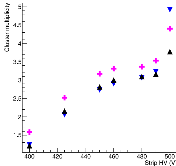
Fig. 20. Cluster multiplicity in 3 FMT disks as a function of HV on the strips.
