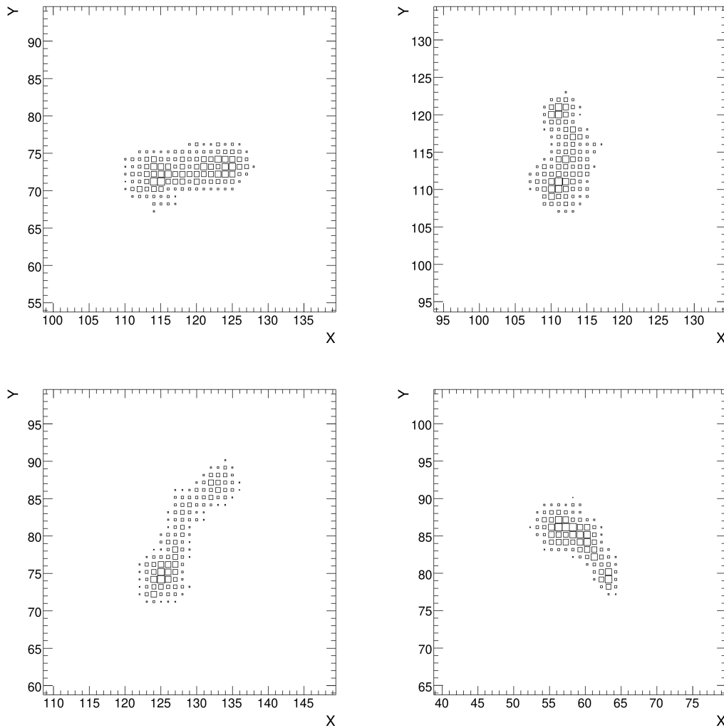
Figure 6.10: Examples of photoelectron tracks ( \simeq 1 mm) obtained with the 5.9 keV x-rays from ^{55}\text{Fe} in Neon(90%)-Isobutane(10%) and a drift distance of 5 mm. The area of each square is proportional to the charge collected by the corresponding pixel set in TOT mode. The size of each image is 2.2 \times 2.2 \text{ mm}^2 ( 40 \times 40 pixels).
