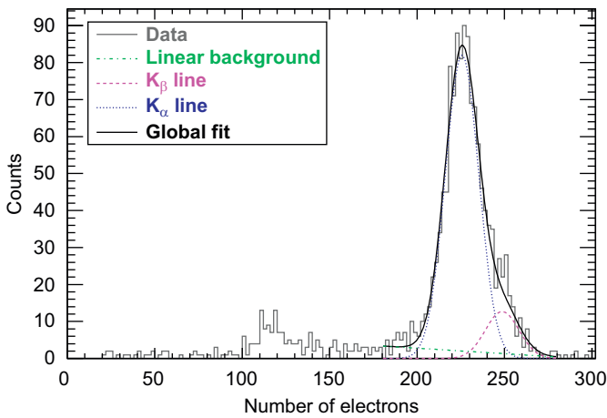
Fig. 3. Spectrum of the number of electrons obtained with each of 2000 photons from 55 Fe source converted in Argon(95%)–Isobutane(5%) gas mixture. The K_{\alpha} and K_{\beta} lines have been fitted by two Gaussians. The mean of the line is 226 electrons and the RMS \approx 4\% . The electron transverse diffusion coefficient was D_t = 500 \mu\text{m}/\sqrt{\text{cm}} at 500 V/cm.
