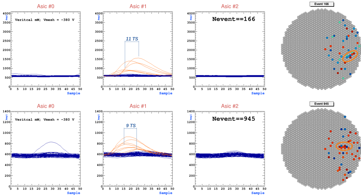
Figure 4. Two examples of muons registered in the Micromegas test bench. The three plots on the left shows the registered signals in each ASIC, corresponding to each sector of the Micromegas. Signals in orange are those over an arbitrary threshold. Time difference between pulses provides information about the track direction in the coordinate perpendicular to the Micromegas plane. Plots on the right show the pads corresponding to the signals over threshold. Due to the multiplexing the triggered pads are 7 times the triggered pulses. However a single continue track is identifiable (circled in orange) corresponding to the muon track projection on the Micromegas plane.
