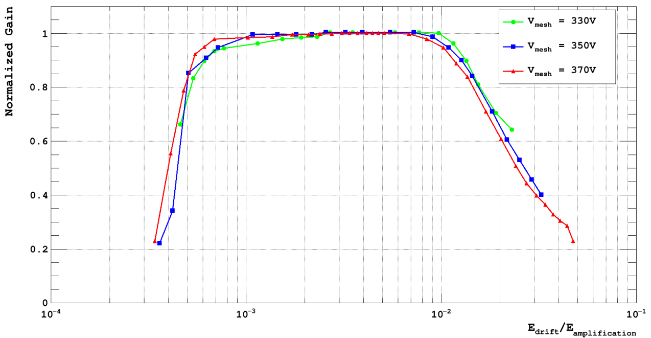
Figure 3.9: Electron transmission in a Bulk Micromegas in T2K gas mixture at various mesh voltages (gain).
