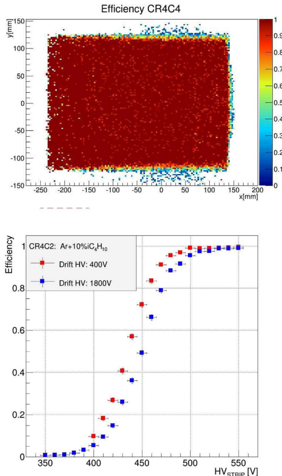
Fig. 13. Efficiency plateau (bottom) and 2D efficiency map (top) for a C-type barrel detector.
