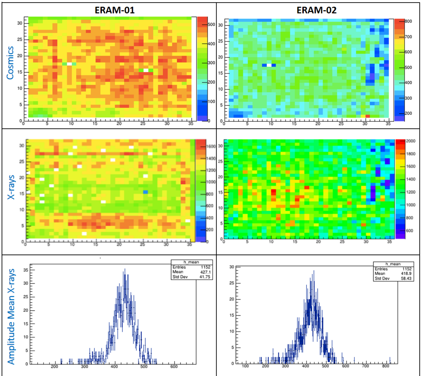
Figure 5.49: Gain maps of ERAM01 and ERAM02 taken from cosmic and X-ray data.
