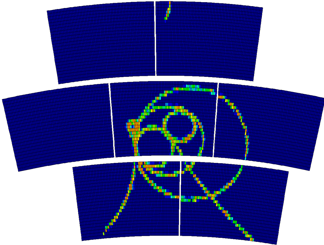
Figure 5.14: Picture of 4 GeV electron beam event recorded by the 7 modules (Run 3036, evt 164).
