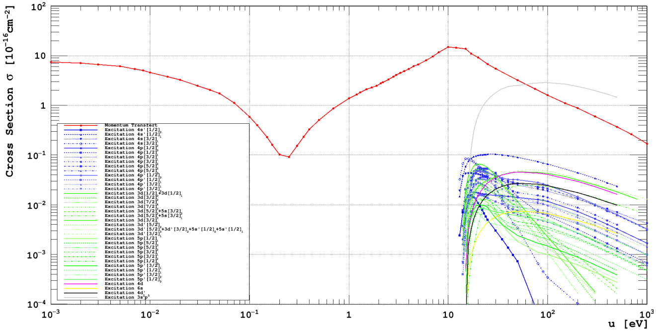
Figure 2.6: Electron cross section with elastic (red) and inelastic (other colors) contributions for argon, based on recent experimental measurements see [6].
