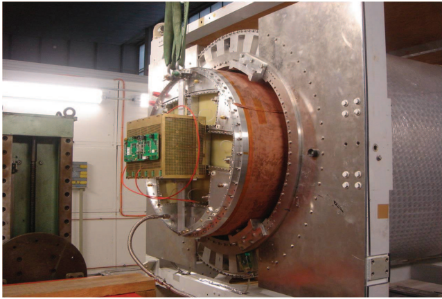
Figure 1. The TPC large prototype and AFTER electronics is pulled out from PCMAG (left figure). View from inside the TPC of the Micromegas module mounted in the middle of the endplate (right figure). Six other modules are dummy.
