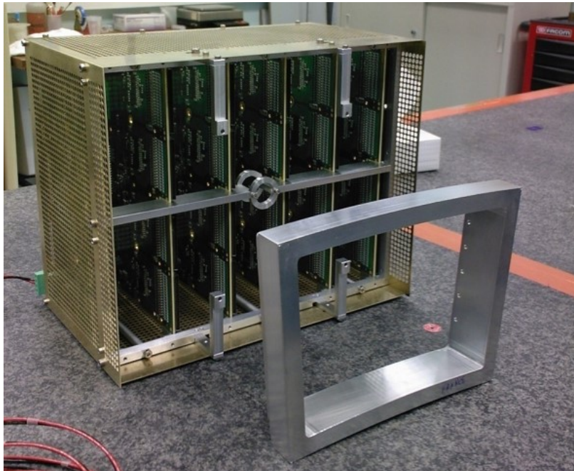
Figure 5.8: Original T2K electronics with light shielding in from of a mechanical frame.
