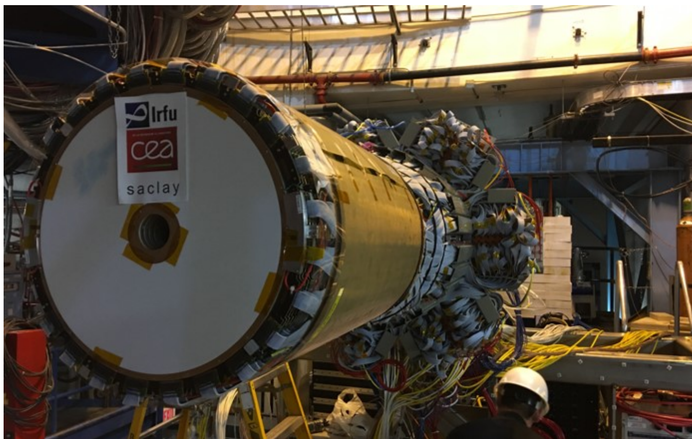
Figure 5.41: Micromegas Central Tracker and Silicon Vertex Tracker during installation at Hall B of Jefferson Laboratory in October 2017.
