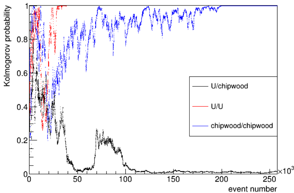
Figure 8.4: Kolmogorov probability in function of the accumulated event number in three different configurations. Taken from [15]
