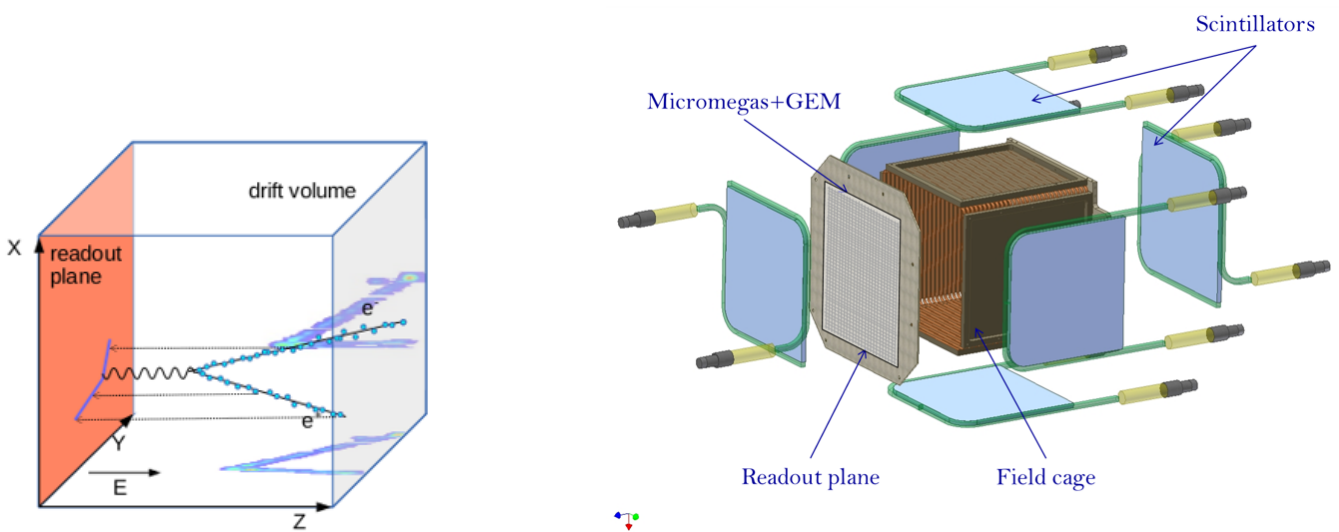
Figure 6.1: [Left] Cubic TPC principle with 2 \times 1\text{D} (x,y)+z readout for 3D tracking. [Right] Description of HARPO TPC prototype.
