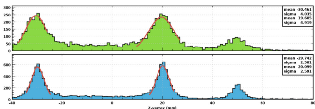
Fig. 28. Preliminary vertex position along the beam axis reconstructed with the SVT-stand-alone reconstruction (top-green distribution) and the CVT reconstruction (bottom-blue distribution) for an empty-target and no solenoid field. The target walls are located at -30 and 20 mm with gaseous hydrogen in-between. At 50 mm, the scattering chamber endcap is clearly visible. The improvement in the resolution from the SVT to the CVT reconstruction is mainly due to the BMT-C tiles.
