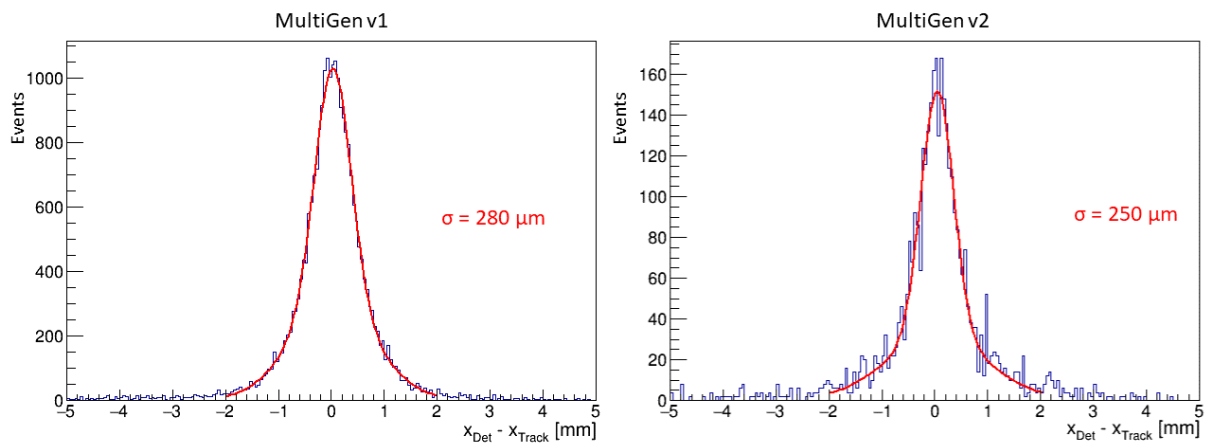
Figure 8.10: Spatial resolution given by distribution of measured position compared to muon track position for MultiGen v1 [left] and v2 [right] in Ar- iC_4H_{10} gas mixture.
