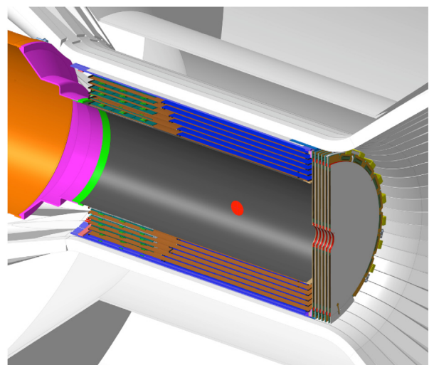
Fig. 2. Cut view showing the 6 different layers of the BMT and the 6 identical FMT disks. The detectors are inserted close to the Central Time-of-Flight, itself in the 5 T solenoid magnet. The SVT is inside the MVT and is not displayed in this view where the beam enters from the left. The red dot indicates the nominal target position. (For interpretation of the references to color in this figure legend, the reader is referred to the web version of this article.)
