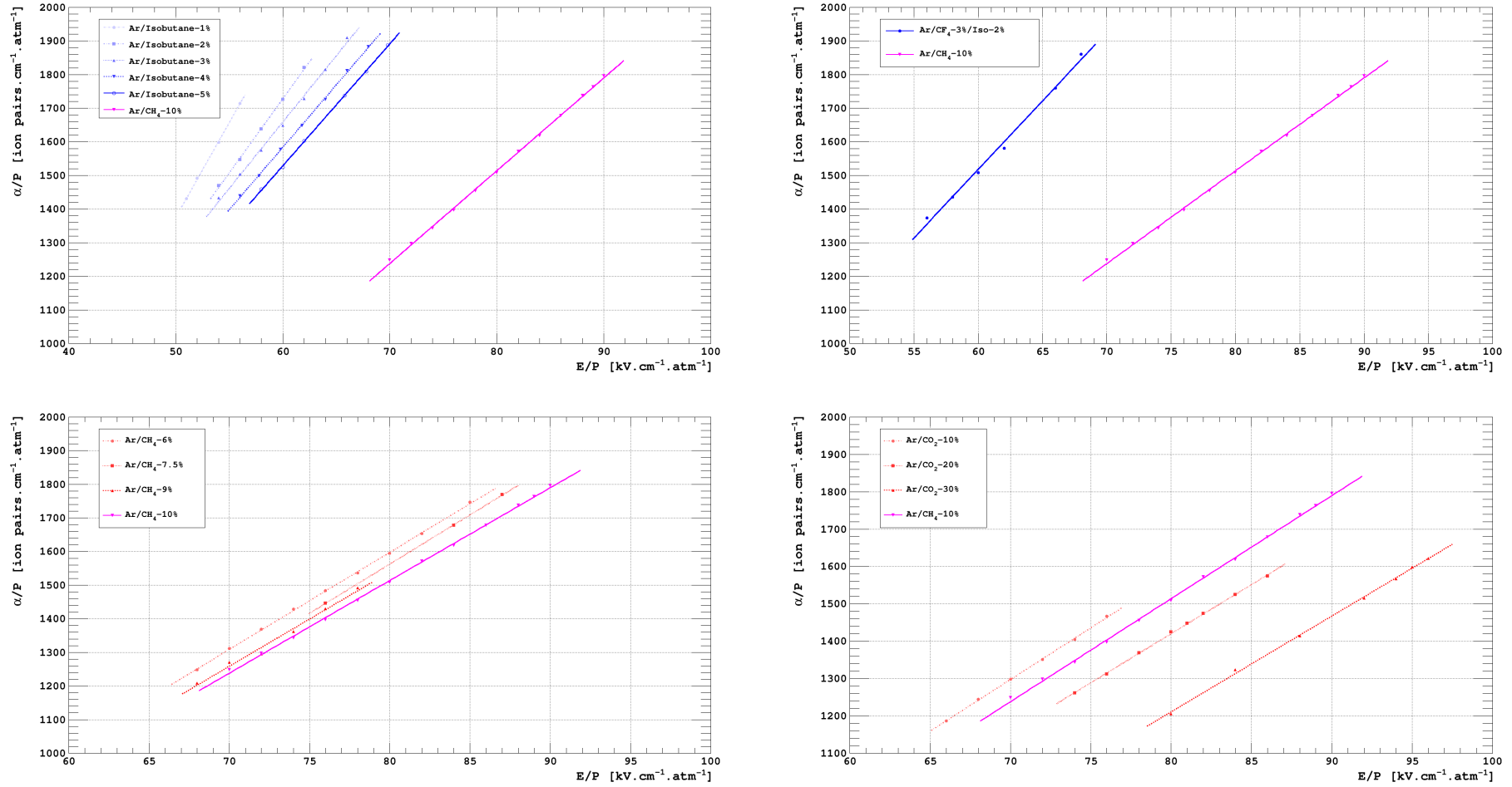
Figure 3.10: Extraction of the Rose and Korff coefficients for [Top left] argon and isobutane mixtures, [Top right] the T2K gas mixture, [Bottom left] for argon and CH 4 mixtures and [Bottom right] for argon and CO 2 mixtures. The argon/CH 4 -10% is shown as reference.
