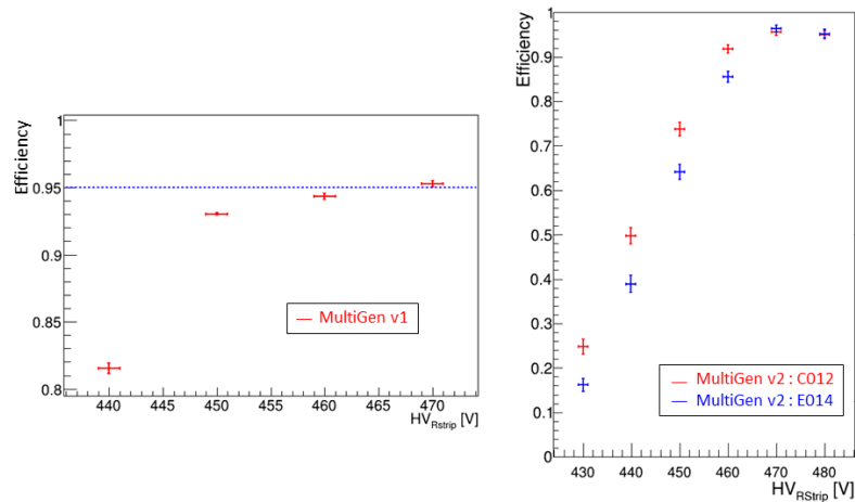
Figure 8.9: Efficiency for MultiGen v1 [left] and v2 [right] in Ar- iC_4H_{10} gas mixture.
