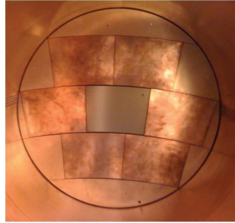
Figure 1. The TPC large prototype and AFTER electronics is pulled out from PCMAG (left figure). View from inside the TPC of the Micromegas module mounted in the middle of the endplate (right figure). Six other modules are dummy.
