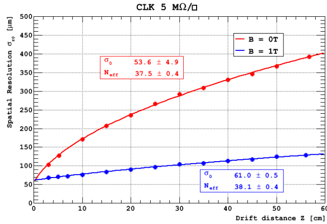
Figure 5.23: Spatial resolution with magnetic field (1 T) in blue and without magnetic field in red for CLK Micromegas.
