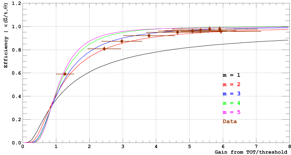
Figure 3.15: Detection efficiency with theoretical curves for Polya distributions with various \Theta parameters and data points. The error on TOT is assumed to be 20%.
