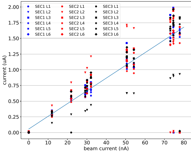
Fig. 22. Currents on the BMT strips as a function of beam current on a 5-cm-long liquid-hydrogen target. All detectors have similar currents. The nominal luminosity of 10^{35} \text{ cm}^{-2} \text{ s}^{-1} corresponds to 75 nA on target.
