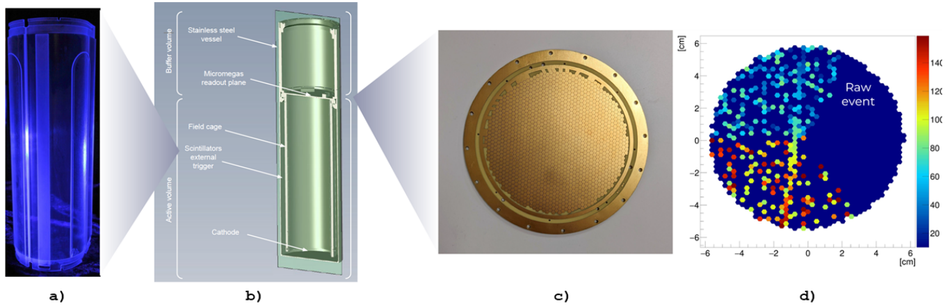
Figure 8.23: CAD 3D drawing of D3DT design (b). (a) View of the cylindrical-shaped scintillator placed between the field cage and stainless steel vessel to provide an external trigger and timing information. (c) Readout plane with its 1344 multiplexed hexagonal pixels for signal readout.
