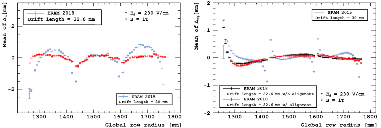
Figure 5.29: Distortions B=1T with beam around z \simeq 3 cm. [Left] Residuals \Delta_z and [right] residuals \Delta_{r\phi} for DLC resistive Micromegas of 2015 in blue and 2018 in red with alignment (and without alignment in black).
