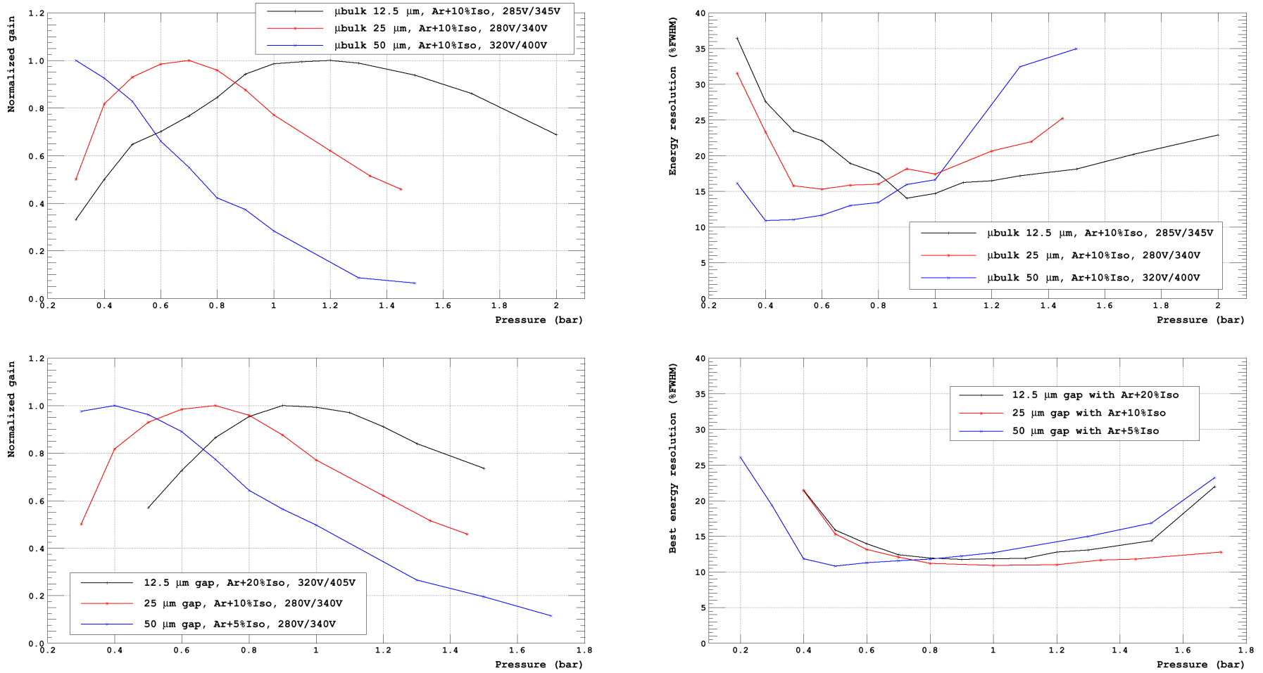
Figure 3.7: Top: normalized gain [left] and energy resolution [right] in function of the pressure for the 12.5 \mu\text{m} , 25 \mu\text{m} and 50 \mu\text{m} gap Microbulk in argon + 10% isobutane gas mixture. Bottom: normalized gain [left] and energy resolution [right] in function of the pressure for the 12.5 \mu\text{m} , 25 \mu\text{m} and 50 \mu\text{m} gap Microbulk in a specific gas mixture with argon and isobutane.
