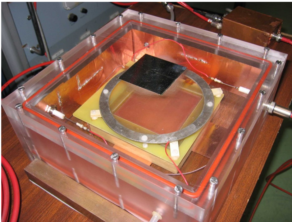
Figure 3.2: Transparent box test with a 50 \mu\text{m} gap copper mesh Micromegas used for the systematic gain measurements.
