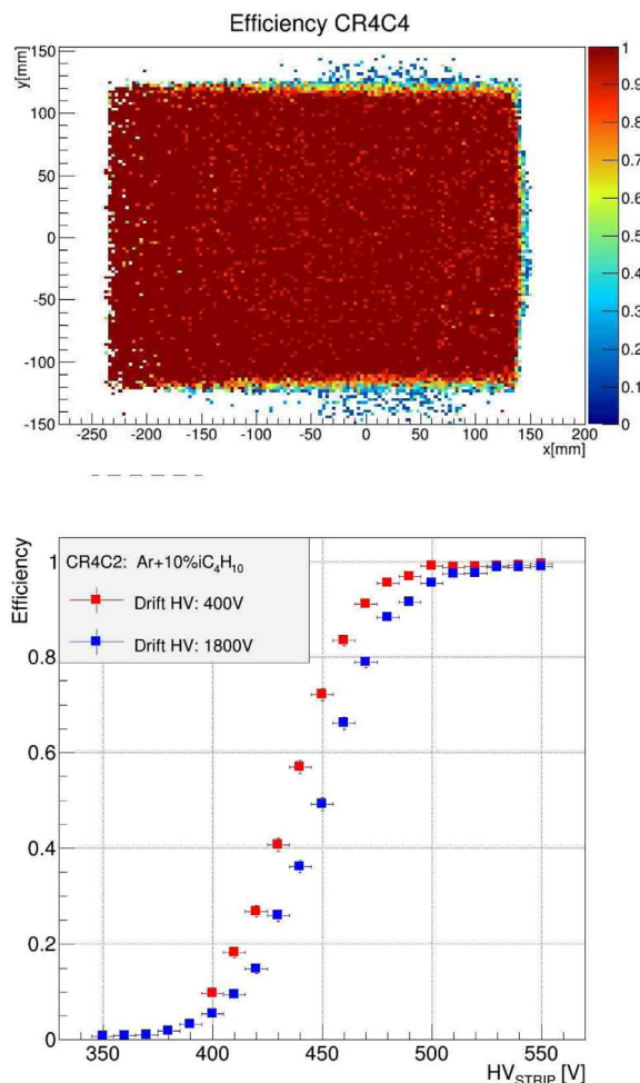
Fig. 13. Efficiency plateau (bottom) and 2D efficiency map (top) for a C-type barrel detector.
