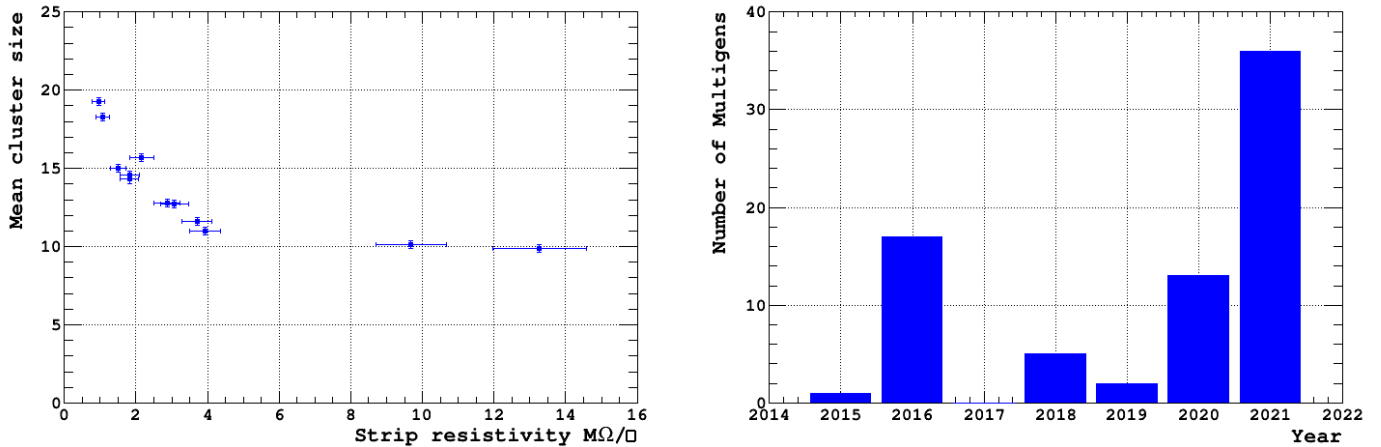
Figure 8.12: [Left] Cluster in function of the strip resistivity. [Right] Production of MultiGen at Elvia-PCB company during the past year.
