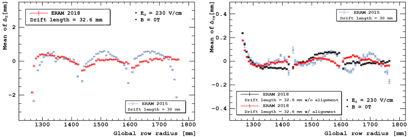
Figure 5.28: Distortions B=0T with beam around z \simeq 3 cm. [Left] Residuals \Delta_z and [right] residuals \Delta_{r\phi} for DLC resistive Micromegas of 2015 in blue and 2018 in red with alignment (and without alignment in black).
