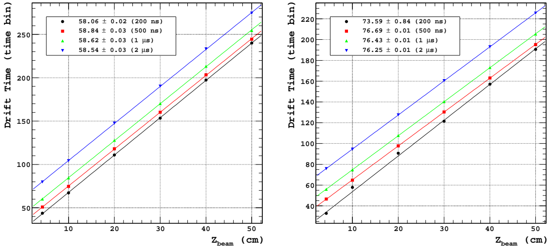
Figure 3. Determination of drift velocities (in \mu\text{m}/\text{ns} ) for several electronics peaking times for two drift field conditions: low drift field condition (140 V/cm) on the left figure and standard drift field condition (230 V/cm) on the right figure. Each time bin is 40 ns for a sampling frequency of 25 MHz.
