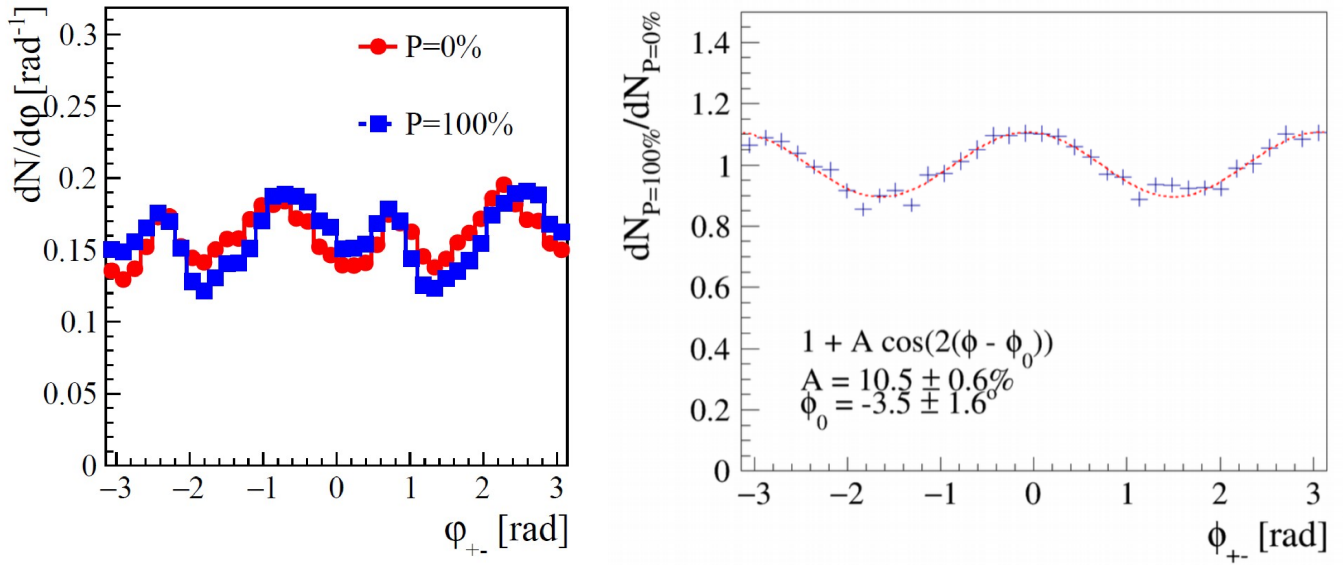
Figure 6.5: Polarisation plots from 11.8 MeV \gamma with HARPO TPC oriented at 0^{\circ} around the beam axis: [Left] distribution of \Phi_{\pm} extracted from data of polarised and unpolarised beam in blue squares and red dots respectively. [Right] Ratio of the azimuthal angle distributions for polarised (P=100%) and unpolarised (P=0%). The systematic bias is cancelled by dividing the azimuthal angle distribution for polarised photons by the distribution for unpolarised photons from experimental data.
