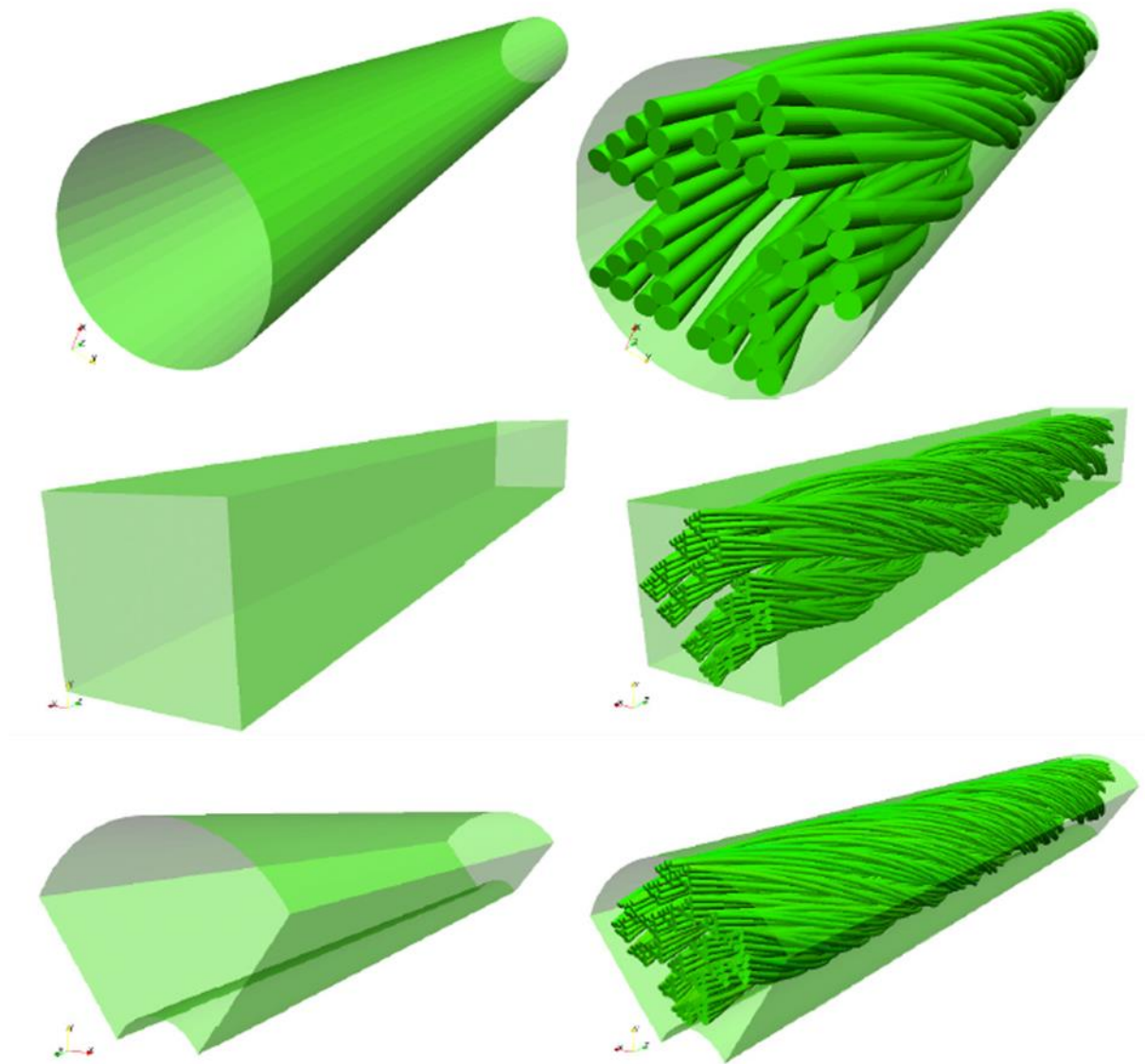
Figure III.2.11. Different shapes of the wires assembly simulated by MULTIFIL thanks to the rigid tools (Bajas 2011).
