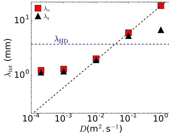
Figure 4.11: \lambda_{n,\text{int}} and \lambda_{q,\text{int}} for \nabla B -drift simulations as a function of the diffusion coefficient in anisothermal JET-like simulation (a)
