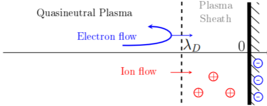
Figure 2.2: Scheme of the sheath region and the quasi-neutral plasma
