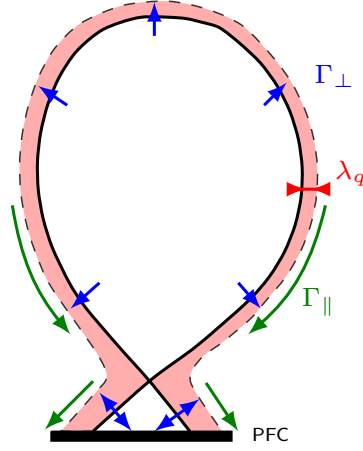
Figure 1.5: Scheme of the SOL width
