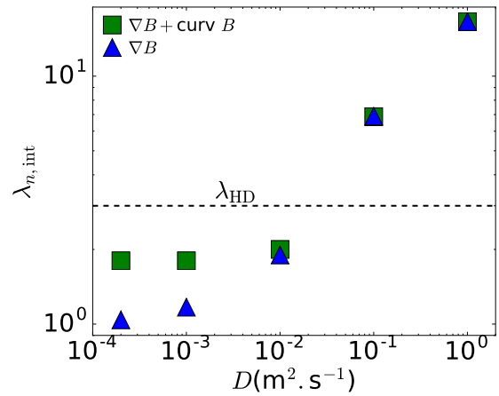
Figure 4.15: \lambda_{n,int} SOL for \nabla B -drift simulations (blue triangles), and \nabla B and centrifugal drift simulations (green squares) as a function of the diffusion coefficient for JET-like simulation
