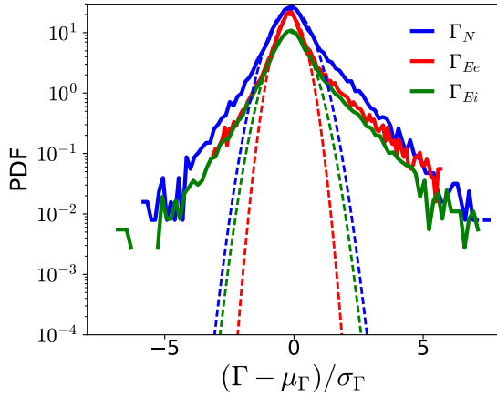
Figure 5.8: PDF of particles and energy turbulent flux in anisothermal simulations at the outer mid-plane and at the radial location r/a = 1.1 a Gaussian fit of the PDF is reported in transparent. PDF are reported in log scale, centered on zeros, normalized by standard deviation
