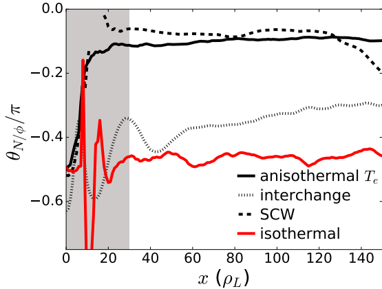
Figure 3.8: Radial profile of \delta_{N/\phi} for isothermal, T_e , pure interchange, and pure SCW simulations, for \sigma = 1 \times 10^{-4} , g = 8 \times 10^{-4} , \zeta = 5 . The radial extent where the turbulence is fully developed in all type of simulations is depicted by the white area, whereas the grey zones correspond to the zone of influence of the source
