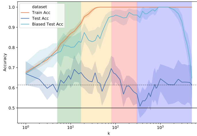
Figure 2.4: Accuracies on training and testing (measured with a 10 folds CV) data as a function of an increased number of ( k ) selected features, using a univariate filter. The "Test Biased" curve shows biased performances obtained with feature selection performed outside of the CV loop, i.e., on all data. The classifier is a linear SVM with C = 1 . The shades surrounding the lines depict the 95% confidence intervals (CIs). The black horizontal lines show the chance level (plain line) and the predictive performances without the feature selection (dotted line). The colored shaded ranges of k depict the four phases of feature ranking: (i) green: improvement, (ii) yellow: instability (iii) red: overfitting, and (iv) blue: neutral effect.
