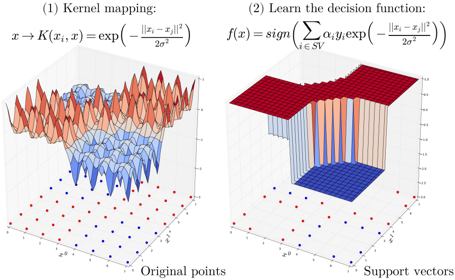
Figure 1.3: Left: Kernel mapping using Gaussian kernel from red and blue dots (lower) to kernel space (upper). Right, Support Vector Machines decision function on the top and support vector on the bottom.
