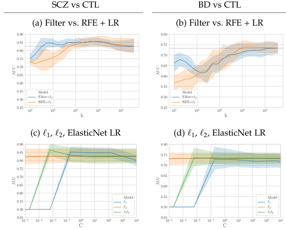
Figure 2.10: Sensitivity analysis: AUC as a function of model complexity parameter for two datasets, left column: SCZ vs. CTL, right column BD vs. CTL. (a, b) AUCs of Filter vs. RFE + \ell_2 regularized Logistic Regression (LR) as a function of k the number of selected features. (c, d) AUCs of \ell_1 (Lasso) vs \ell_2 vs. ElasticNet- regularized LR as a function of the regularization parameter C . The dotted horizontal line provides the baseline performance of a \ell_2 regularized LR with C = 1 .
