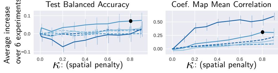
Figure 4.1: Sensitivity analysis of the spatial penalization parameter averaged across 6 experiments: the 3 datasets for both 3D GM and cortical thickness. Y-axis reports the differences of score (balanced accuracy in left panel or map stability in right panel) with the baseline ElasticNet that are averaged across the experiments for an increased spatial penalty in TV (plain lines) or GN (dashed lines). The models Eq. 4.1 and Eq. 4.2 were re-parameterized with only two parameters: \alpha which determines the global penalty and \kappa which controls the ratio of \ell_2 over the spatial penalty. The ElasticNet penalty has a fixed \ell_1/\ell_2 ratio of 0.1 with \lambda_1 = \alpha/10 and \lambda_2 = \alpha . Finally, \lambda_{s \in \{TV, GN\}} = \alpha\kappa with \kappa \in [0, 1] . The darkness of blue lines codes for the global strength of the penalty: dark \alpha = 1 , medium \alpha = 0.1 , and light blue \alpha = 0.01 . Left panel: the balanced accuracy. Right panel: stability of the coefficient map as the average correlation (using Fisher’s z-transformation) between pairs of coefficient maps computed across the 5 CV-folds.
