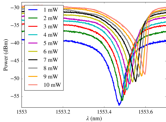
(a) Optical spectra for increasing laser powers.
