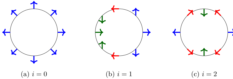
Figure IV.11 – Mode shape of the i = 0, 1, 2 extensional vibrational modes.
