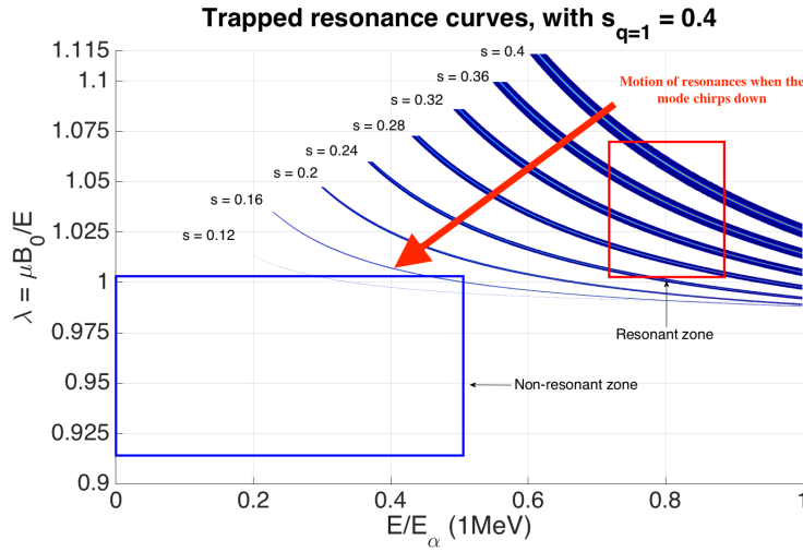
Figure 6.5: Positions of the precessional resonance on the (E, \lambda) diagram for trapped particles, at different radii. Two zones are identified, a zone free from resonances (blue) and one crossed by many resonances (red). When the MHD mode frequency chirps down, the resonant curves are displaced at lower energies and pitch angles.
