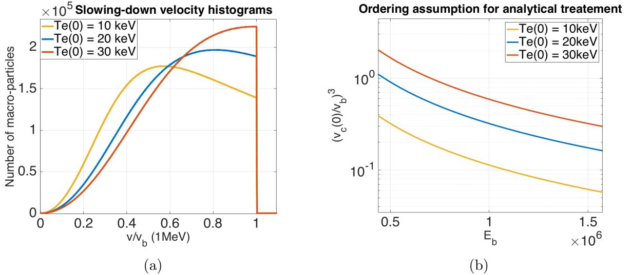
Figure 5.7: (a) Velocity histogram of slowing-down distribution functions for different on-axis electron temperature. (b) Cubic ratio between the critical velocity and the birth velocity, as a function of the birth energy for different on-axis electronic temperatures
