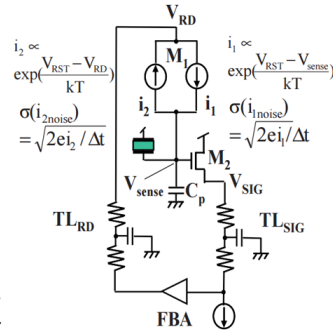
Fig. 3 Equivalent circuit of noise canceller.
