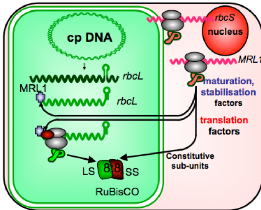
Figure 12. The role of MRL1 in stabilising and enhancing translation of the mRNA for the large subunit of Rubisco in Chlamydomonas and Arabidopsis .
