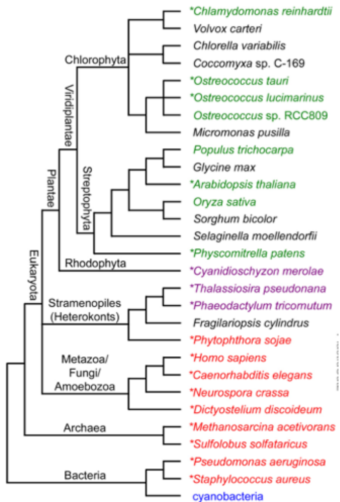
Figure 15. Chlamydomonas reinhardtii is haploid, and has a nuclear genome comprising 17 chromosomes with a total size of ~120 Mbp, with 14 400 coding genes. By comparing these genes against the genes of other sequenced species in green and red Chlamydomonas appeared to have a genetic makeup composed of both plant and animal genes. Genes that were present in the green lineage genomes and always absent in non-green lineage make up the green cut: 597 conserved proteins that may function in the chloroplast. Interestingly, more than half of these have of an unknown function, so as potential candidates for photosynthetic regulators they have enormous potential and because this analysis is conservation-based it's not only a tool for algae but for plants as well.
