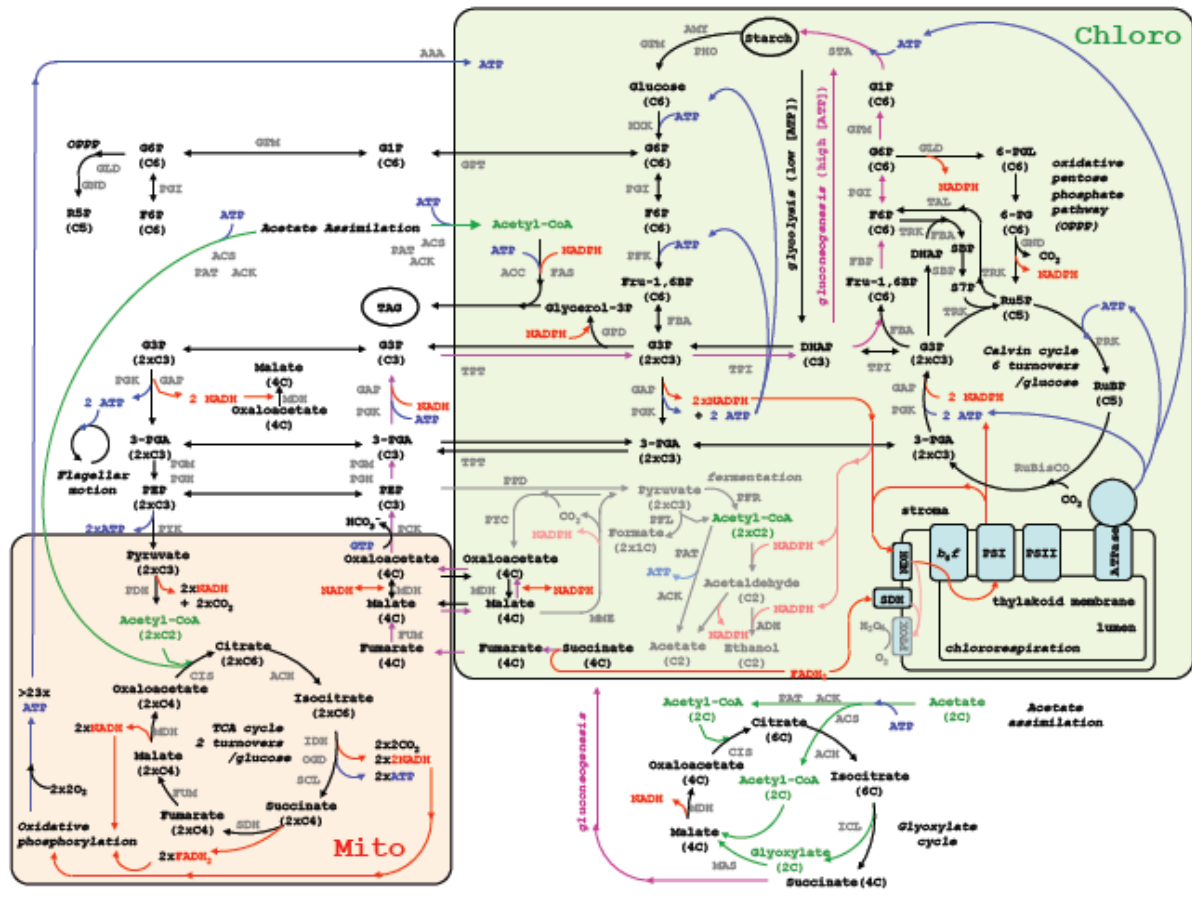
Figure 23. Shows the complex interaction between the phototrophic and respiratory energy budget of ATP and NAD(P)H in Chlamydomonas . Special attention has been placed on the expected compartmentalization of these reactions [79].
