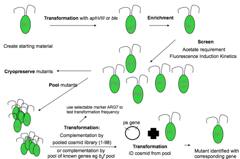
Figure 10. Schematic representation of a medium-flow functional genomics technique to isolate biogenesis factors of the photosynthetic complexes.
