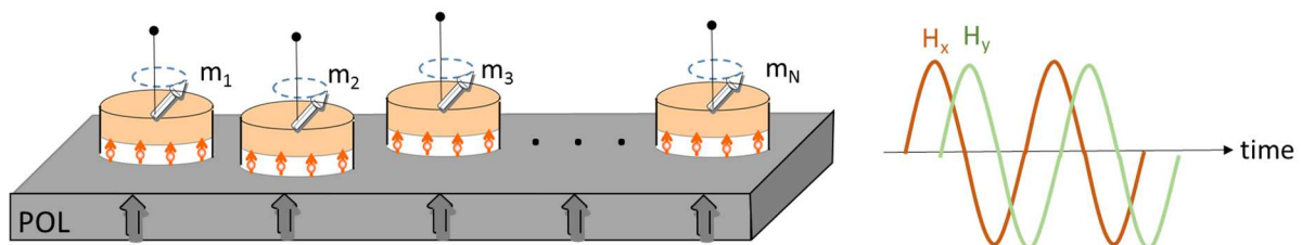
Fig. 5.5 a) Chain of synchronized STNOs aimed at generating a RF stray field in free space. They consist of a perpendicular polarizer ( [\text{Co/Pt}]_n/\text{Co} ) and an in-plane magnetized free layer separated by a non-magnetic Cu spacer. All the STNOs are traversed by a perpendicular DC current which generates a large angle precession of the free layer magnetization by STT.
