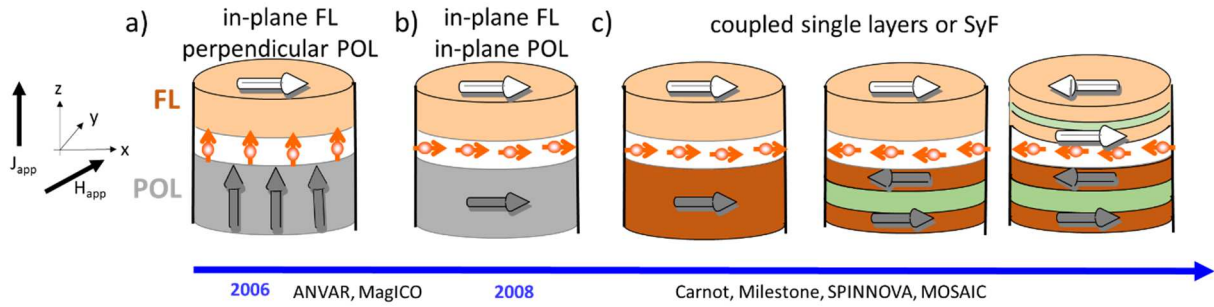
Fig. 3.2 Schematics of typical STNO nanopillar structures. The free layer magnetization (FL) is laying in xOy plane while the magnetization of the reference layer (polarizer POL) is fixed either perpendicular to plane (a) or in the plane of the dot (b). c) The polarizer might be free to evolve being coupled to the free layer, or even replaced by a synthetic anti-ferromagnet. Bottom : time scale of STNO topic at Spintec and the associated grants.
