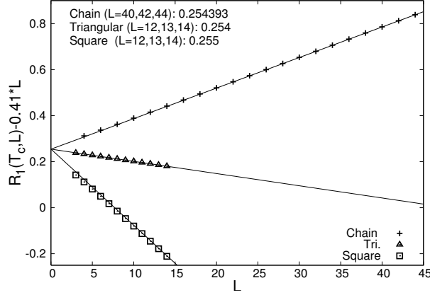
Figure 2.5: Shannon entropy of three Ising models at the critical point, plotted as a function of L (a linear term, -0.41L , has been subtracted for clarity). Data for the 2D square and 2D triangular lattices and for the ICTF are compared. The entropy is well fitted by \simeq aL + r_1 + b/L and the subleading constant r_1 is evaluated using the three largest sizes. Taken from [4].
