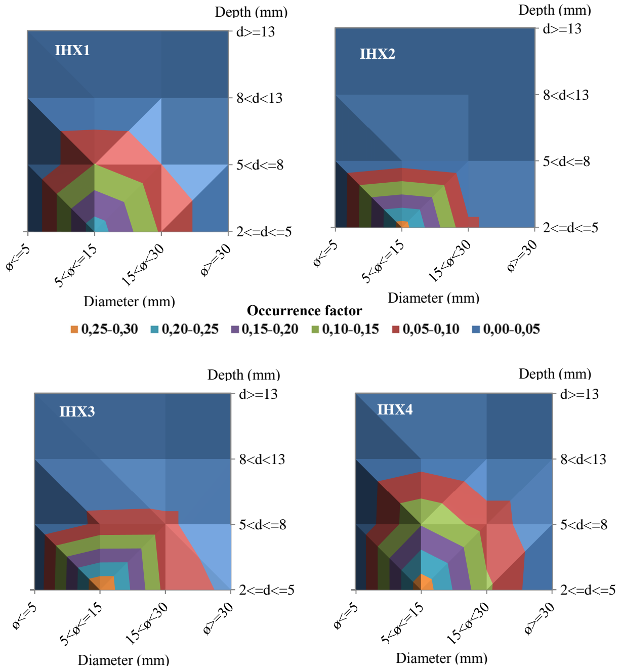
Fig. 10 Occurrence factor depending on the vortex depth ( d in mm) and diameter at mid-depth ( \phi in mm) at the water nominal level.
