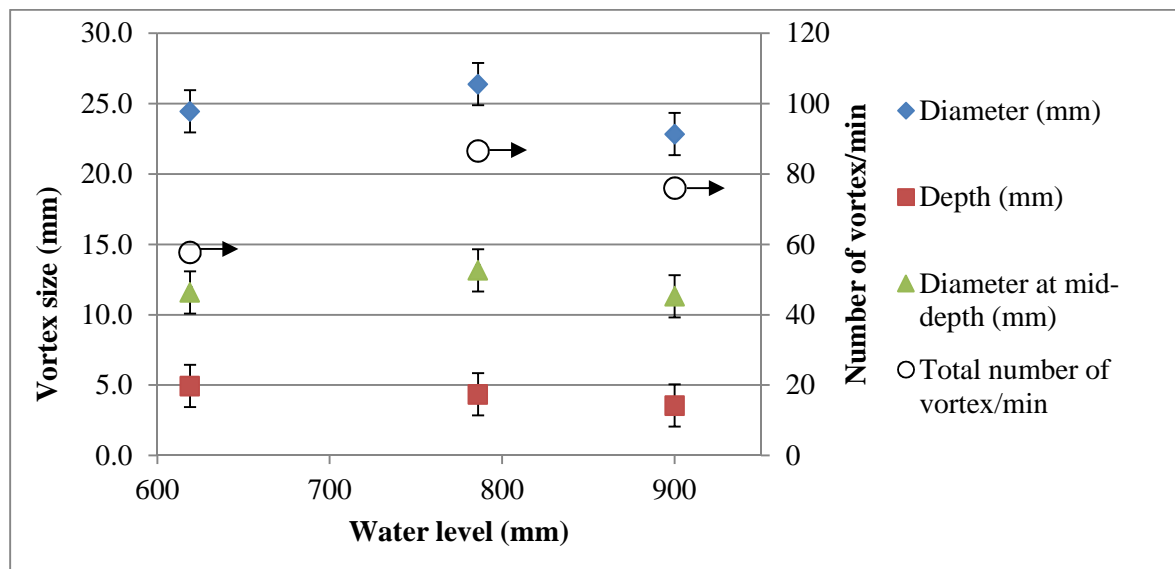
Fig. 7 Size and amount of vortices around the 4 IHX depending on the water level.
