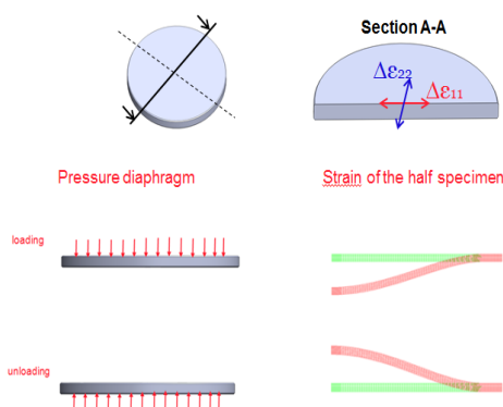
Figure 1. Principle of the new experimental fatigue test.
