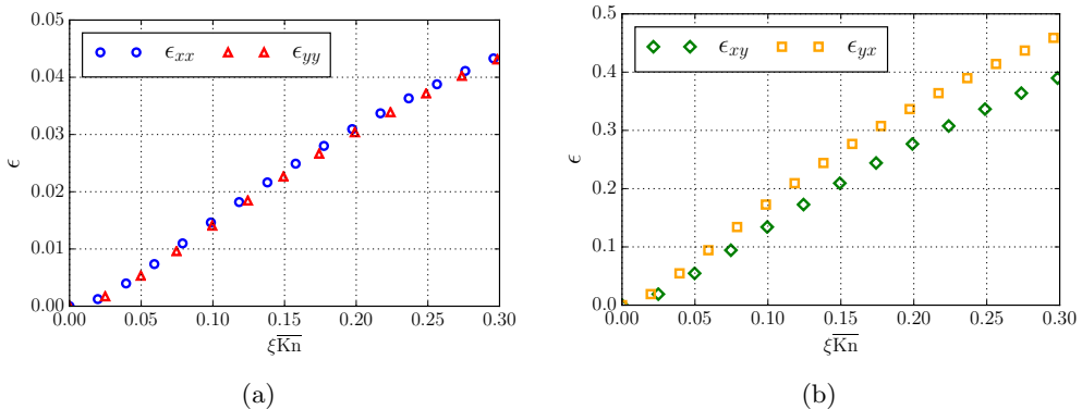
Figure 9: Evolution of the relative error between the computed solution of the complete closure problem (3.33) and estimated at the first-order with the solutions of the sub-problems (3.46) and (3.47). The solution of the complete closure problem is taken as the reference: a) diagonal components; b) extra-diagonal components.
