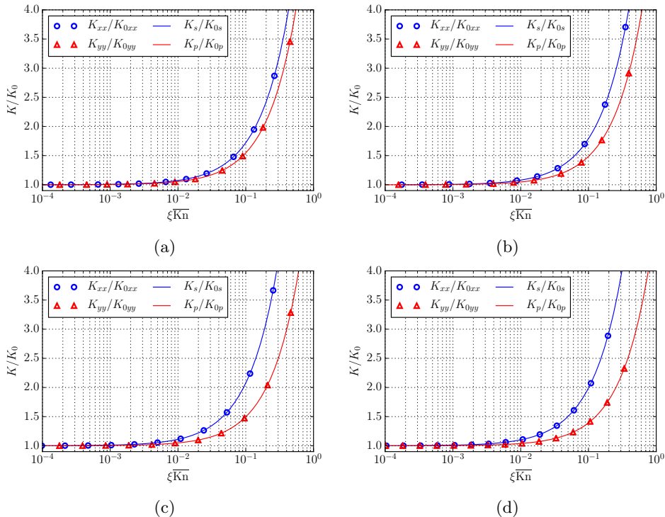
Figure 4: Ratio of the apparent slip-corrected to intrinsic transmissivity K_{ij}/K_{0ij} as a function of \xi\bar{K}\bar{n} = \xi\bar{\lambda}/h_{\beta j} for the sinusoidal fracture defined by equation (4.3) (a) #1, c) #3) and the exponential aperture field given in equation (4.11) (b) #1, d) #3) (see parameters for aperture fields #1 and #3 in table 1). The characteristic aperture h_{\beta j} is defined by the relationship (4.18). Dots represent the solutions computed from the closure problem (3.33) while solid lines are the analytical solutions reported in equations (4.4), (4.8) and (4.13), (4.14).
