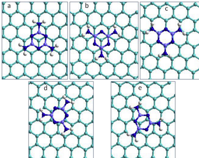
Fig. 1. Optimized structures of melamine on different adsorption sites upon graphene: topC-top (a), N-top (b), All-top(c), cross (d), bridge (e). Graphene carbon atoms are in cyan, nitrogen in blue, hydrogen in white, carbon of melamine in lilas. (For interpretation of the references to colour in this figure legend, the reader is referred to the web version of this article.)
