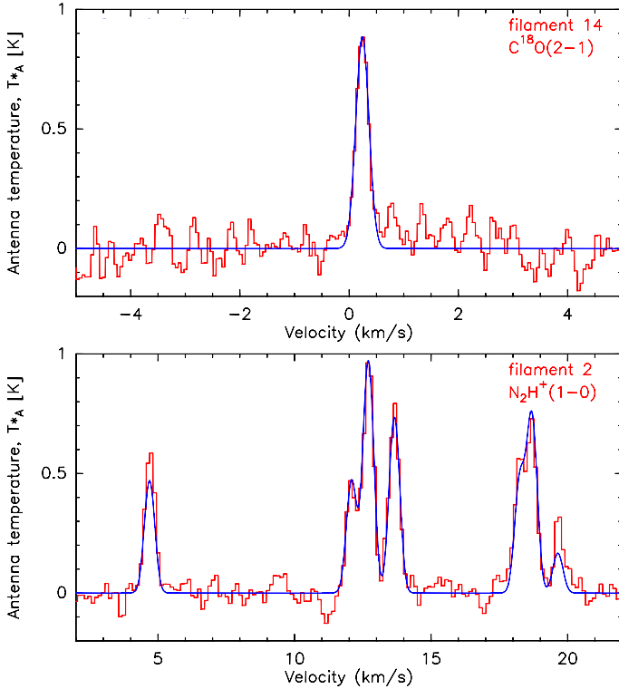
Fig. 2. Spectra observed in the C^{18}O(2-1) and the N_2H^+(1-0) transitions, toward filament 14 ( top ) and 2 ( bottom ), respectively. The best Gaussian fits to the spectra are overlaid in blue. The fitted parameters are given in Table 1.
