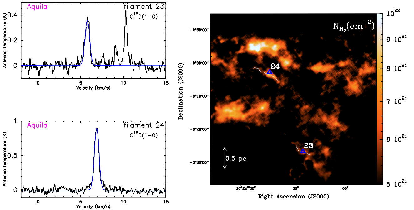
Fig. A.8. \text{C}^{18}\text{O}(1-0) spectra observed toward filaments 23 and 24 in Aquila, located in the south west part of the region. The positions of the two filaments are shown on a blow up of the column density map (cf., Könyves et al. 2010) on the right hand side. Filament 24 shows a single velocity \text{C}^{18}\text{O}(1-0) spectrum at V_{\text{LSR}} = 6.87 \text{ km s}^{-1} , while \text{C}^{18}\text{O}(1-0) spectrum observed toward filament 23 shows three velocity components at V_{\text{LSR}} = 5.77 \text{ km s}^{-1} , 9.13 \text{ km s}^{-1} and 10.3 \text{ km s}^{-1} . The relevant velocity component associated to filament 23 is most probably the component at V_{\text{LSR}} = 5.77 \text{ km s}^{-1} (the closest to the LSR velocity of the neighboring filament 24), while the other components are likely associated to clouds/filaments observed on the same line-of-sight.
