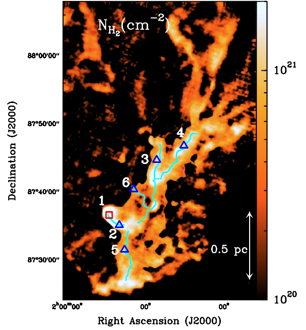
Fig. A.10. Curvlet component of the column density map of a subregion in the Polaris Cloud taken from André et al. (2010). The positions of the observed spectra are plotted in red squares and blue triangles for \text{N}_2\text{H}^+ and \text{C}^{18}\text{O} , respectively. The numbers correspond to the filaments listed in Table 1.
