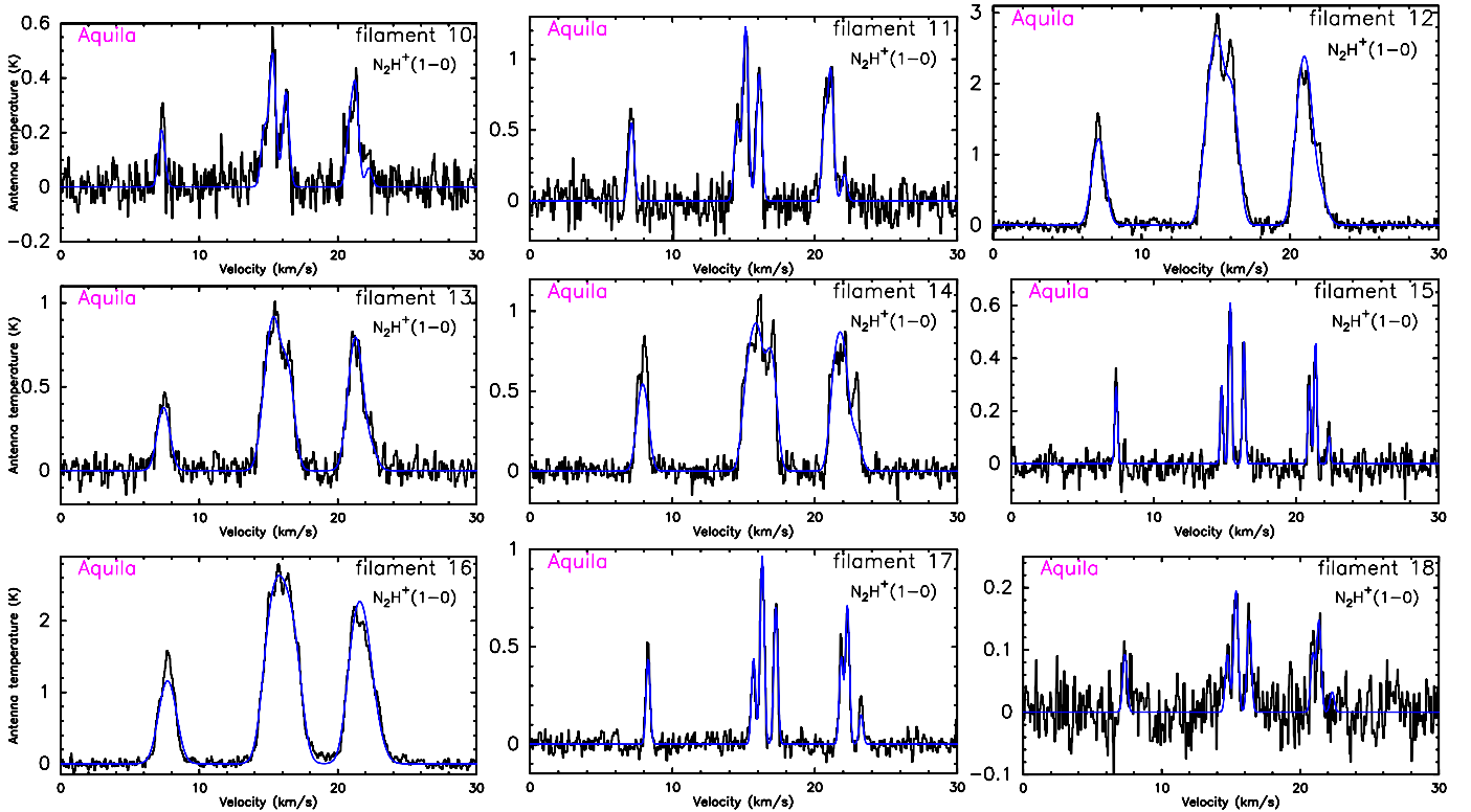
Fig. A.6. Continuation of Fig. A.4 presenting the N_2H^+(1-0) spectra observed toward 9 filaments in Aquila.
