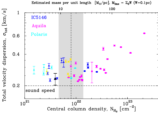
Fig. A.1. Total velocity dispersion versus observed central column density. Similar plot to Fig. 6 for the filaments observed in IC 5146, Aquila and Polaris. The six C^{18}O spectra showing two or three velocity components are flagged in yellow.
