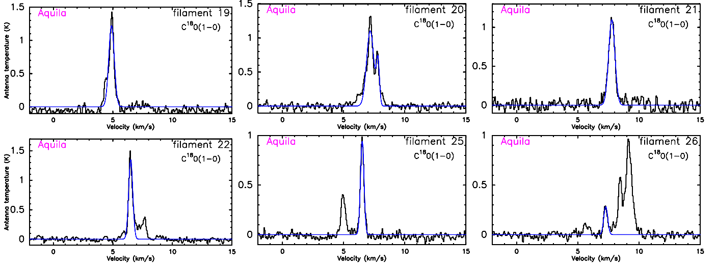
Fig. A.7. \text{C}^{18}\text{O}(1-0) spectra observed toward 6 filaments in Aquila. The corresponding Gaussian fits are highlighted in blue. Note 1: filament 20 shows two components separated by 0.63 \text{ km s}^{-1} . The component at V_{\text{LSR}} = 7.17 \text{ km s}^{-1} have been chosen to be tracing the filament, since this component has a velocity component which is closer to the average velocity ( \bar{V}_{\text{LSR}} = 7.4 \text{ km s}^{-1} ) of the filaments in Aquila which show one velocity component. Note 2: the spectrum observed at the position of filament 22 shows two velocity components, one centered at 6.5 \text{ km s}^{-1} and the other at 7.7 \text{ km s}^{-1} . The strongest component has been selected for similar reasons to that explained for filament 20. Note 3: the spectrum observed at the position of filament 25 has two velocity components (at 5.0 \text{ km s}^{-1} and 6.52 \text{ km s}^{-1} , respectively). The strongest component has been selected for similar reasons to that explained for filament 20. Note 4: the spectrum observed at the position of filament 26 shows three velocity components centered at 7.28 \text{ km s}^{-1} , 8.45 \text{ km s}^{-1} and 9.17 \text{ km s}^{-1} , respectively. The component centered at 7.28 \text{ km s}^{-1} has been selected because it is the component with the closest V_{\text{LSR}} value to the mean \bar{V}_{\text{LSR}} of neighboring filaments in Aquila.
