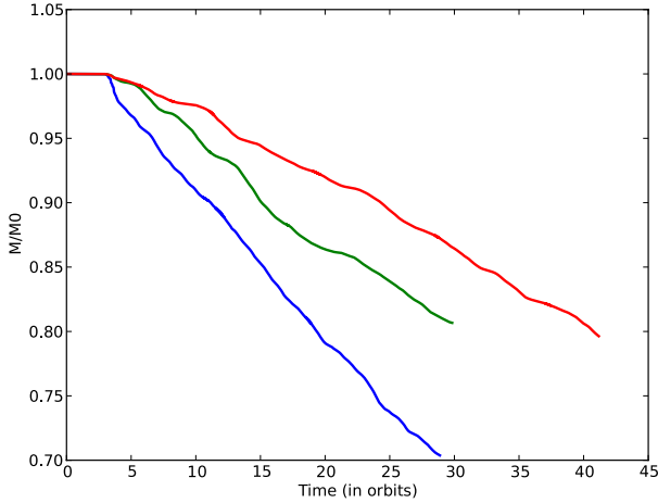
Fig. 2. Time-evolution of the total relative mass in the box when the radial extent of the box is varied from L_x = H (blue line) to L_x = 2H (green line) and L_x = 4H (red line).
