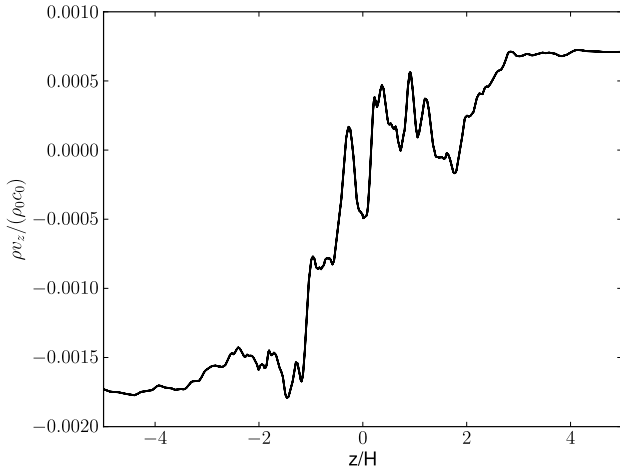
Fig. 8. Vertical profile of the horizontally averaged vertical mass flux, \langle \rho v_z \rangle , obtained in model Diffu4H . The data are time-averaged over a single burst between t = 22 and t = 27 and normalized by \rho_0 c_0 .
