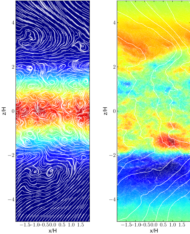
Fig. 7. y -averaged poloidal streamlines (left panel) and poloidal magnetic field lines (right panel) in the (x, z) plane, time-averaged over the ejection event occurring at 22 < t < 27 , and overplotted on the density distribution (left panel) and azimuthal magnetic field distribution (right panel).
