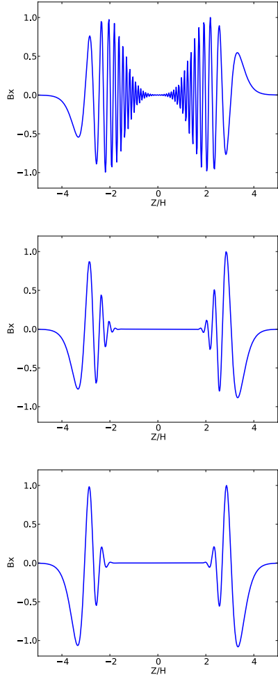
Fig. A.1. Vertical profile of the radial magnetic field eigenmode for three different sets of dissipation coefficients. From left to right, Rm = Re = 10^6 , Rm = Re = 10^4 and Rm = Re = 3000 .
