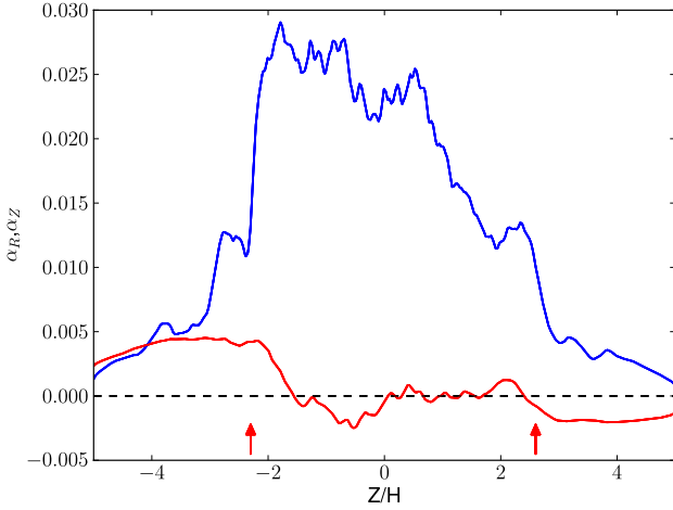
Fig. 14. Vertical profile of \alpha_R (blue curve) and \alpha_Z (red curve), time averaged using the data of model Diffu4H over the interval 22 < t < 27 . Vertical arrows marks the location of unit ratio between horizontally averaged thermal and magnetic pressures.
