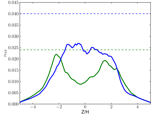
Fig. 12. Vertical profile of the total stress tensor, normalized by the midplane pressure, for models Diffu4H (blue line) and Diffu4HPmhalf (green line). The blue and green dashed lines represent the corresponding values obtained in unstratified runs having the same parameters.
