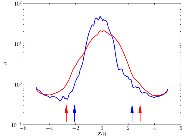
Fig. 3. Vertical profile of the ratio \beta between the horizontally averaged thermal pressure and the horizontally averaged magnetic pressure. The blue curve corresponds to model Diffu1H and results from a further time average between t = 10 and t = 15 orbits. The red curve was obtained averaging the data of model Diffu4H between t = 10 and t = 30 . For each model, the vertical arrows report the approximate wind launching location where \beta = 1 (SI09).
