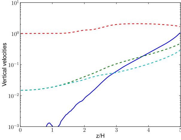
Fig. 13. Same as Fig. 4, but for the model having zero-gradient vertical boundary conditions on B_x and B_y .
