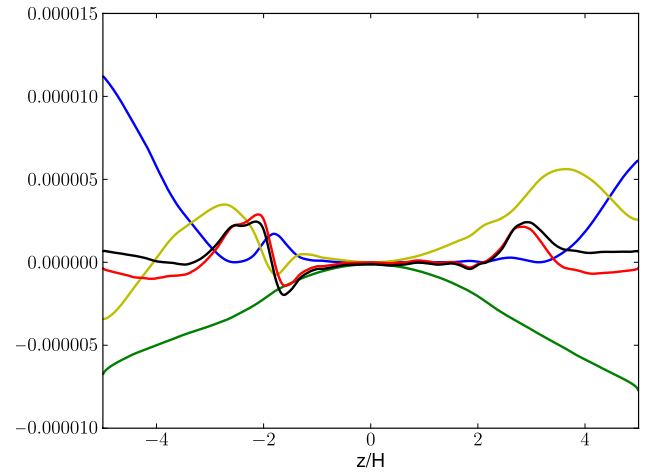
Fig. 10. Vertical profiles of the quantities E_K (blue curve), E_B (red curve), E_T (green curve), E_\phi (yellow curve) and their sum E (black curve) along a particular magnetic field line. Data have been horizontally averaged and time averaged between t = 22 and t = 27 , i.e. over a single ejection event.
