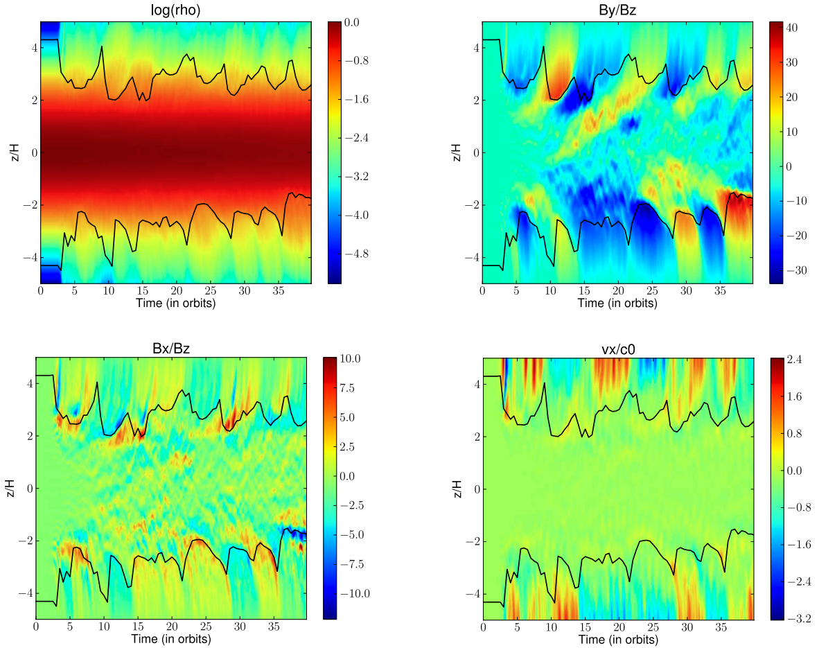
Fig. 6. Space-time diagram of the logarithm of the horizontally averaged mass density ( upper left panel ), \langle B_y \rangle / \langle B_z \rangle ( upper right panel ), \langle B_x \rangle / \langle B_z \rangle ( lower left panel ) and \langle v_x \rangle / c_0 ( lower right panel ) for model Diffu4H . For all panels, the solid line shows the location of unit ratio of horizontally averaged thermal and magnetic pressures, \beta = 1 .
