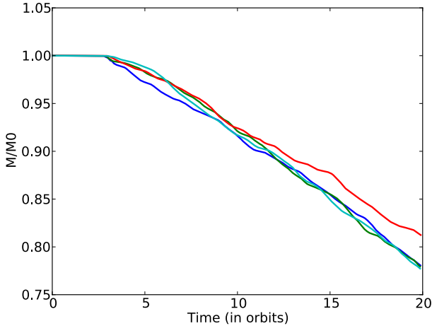
Fig. 1. Time evolution of the total relative mass in the box when the number of cells in the vertical direction is varied: N_z = 256 (blue line), N_z = 512 (green line), N_z = 1024 (red line) and N_z = 2048 (light blue line). All other run parameters are fixed.
