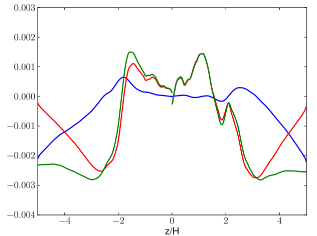
Fig. 11. Vertical profiles of the quantities \mathcal{L} (blue curve), \langle B_y \rangle / \alpha (red curve) and the expected invariant f = \mathcal{L} - \langle B_y \rangle / \alpha (green curve) along a particular magnetic field line, computed as in Fig. 10.
