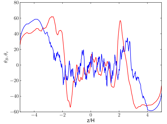
Fig. 9. Vertical profiles of the angles \theta_B (red curve) and \theta_v (blue curve), measured between the vertical axis and the horizontally averaged poloidal magnetic and velocity fields, respectively. Both curves are obtained from model Diffu4H and are time-averaged over a single burst of ejection between t = 22 and t = 27 .
