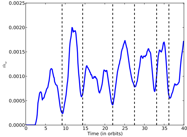
Fig. 5. Time evolution of \dot{m}_w for model Diffu4H (blue curve). The vertical lines mark the times at which the mean toroidal magnetic field at the top boundary of the box changes sign.
