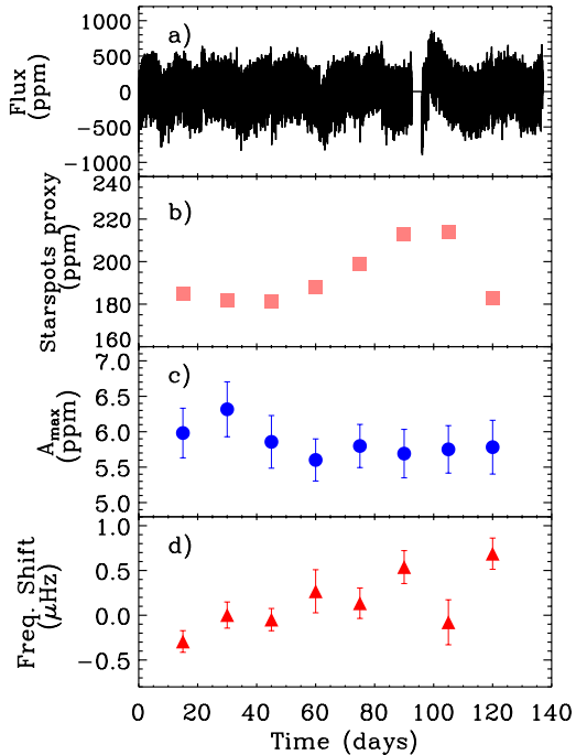
Fig. 2. a) Flux of HD 49385 as a function of time (starting October 18, 2007) measured by CoRoT (only 1 point every 5 has been plotted). b) starspot proxy computed as described in Sect. 2. c) temporal variation of the maximum amplitude per radial mode with their associated error bar. d) temporal variation of the averaged frequency shift of the p modes. In panels b) , c) , and d) , only every other point is independent.
