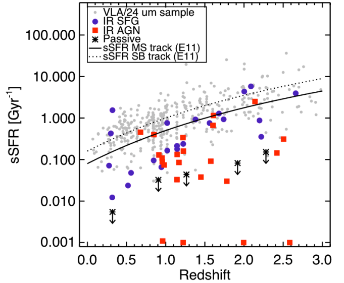
Fig. 10. Specific star formation rate (sSFR) vs. redshift for the entire VLA/24 \mu m sample (grey dots) and for the radio-excess sources, divided into their three IR categories: IR AGN (red squares), IR SFG (blue circles) and passive systems (asterisks). The four sources plotted at the bottom (with a symbolic value of sSFR = 0.001 Gyr -1 ) are the four IR AGN for which the SFR could not be estimated (see Sect. 4.3). The tracks in the plot show the sSFR evolution with redshift for main sequence star-forming galaxies (MS; solid line) and for starburst galaxies (SB; dotted line) from Elbaz et al. (2011). The radio-excess sources have typically lower star formation than the star-forming galaxy population detected at 24 \mu m.
