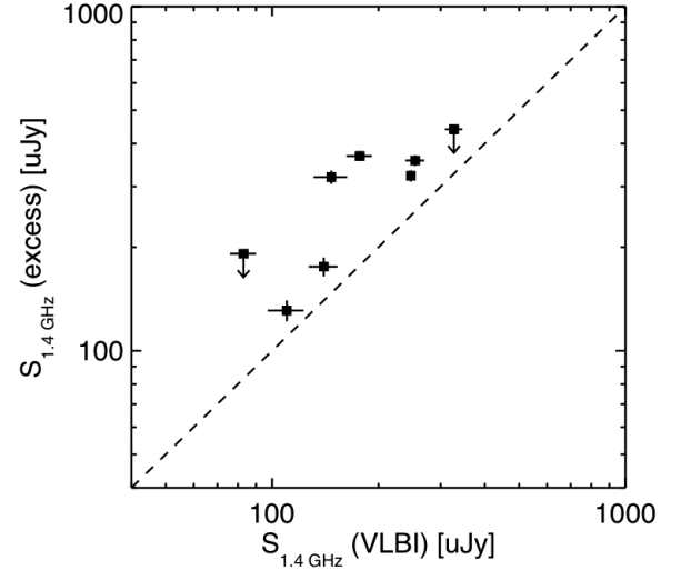
Fig. 8. Radio core flux density at 1.4 GHz measured from the VLBI data (Chi et al., in prep.) vs. the excess radio emission (i.e., S_{1.4 \text{ GHz, tot}} - S_{1.4 \text{ GHz, SFG}} ) for our radio-excess sources. Our radio fluxes agree with the VLBI measurements within a factor \approx 2 ; our fluxes are typically higher because they might include some extended radio emission from outflows, or “aborted jets” (e.g. Ghisellini et al. 2004).
