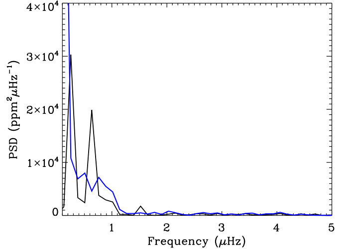
Fig. 4. Low-frequency part of the power spectrum between 0.1 and 5 \mu\text{Hz} . The black line corresponds to the light curve shown in Fig. 2. Two peaks are visible at 0.25 and 0.64 \mu\text{Hz} . The blue line corresponds to the PSD of the light curve in which the jumps at 43.3 and 80.05 days were corrected.
