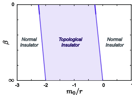
Figure 2: A possible phase diagram of the 3D topological insulator with the “Wilson term” r = 0.5 . It is based on the mean-field calculation around the strong coupling limit ( \beta = 0 ), and extrapolated to the noninteracting limit ( \beta = \infty ).
