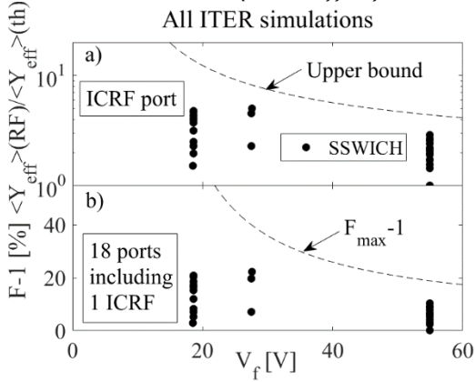
Fig. 5: Enhancement factors for gross W production a) over ICRF port sides and b) over 18 ITER ports, versus floating potential.
