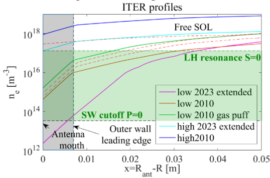
Fig. 2. Density profiles used for the present study versus radial distance to antenna mouth, together with characteristic densities for the slow mode.
