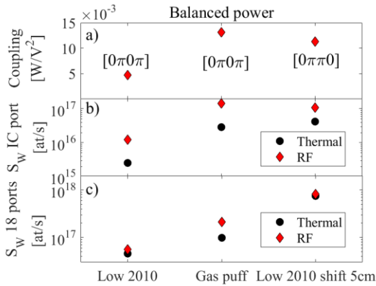
Fig. 7: Comparison of a) RF coupling capability, b) gross W erosion on ICRF port and c) over 18 ports, with or without RF power, using low “Low 2010” (baseline or shifted by 5cm) and “gas puff” density profiles.
