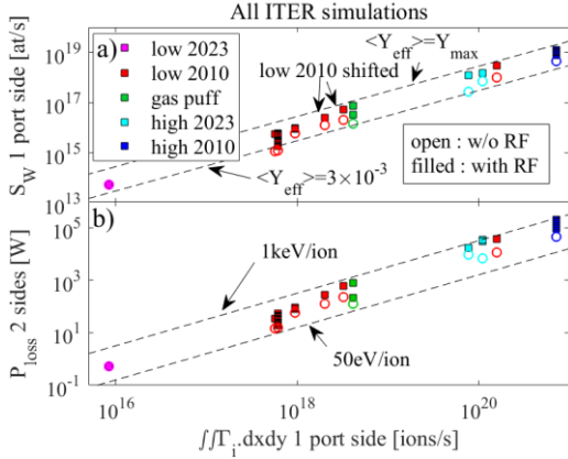
Fig. 3. a) Total gross W source from and b) total power loss onto the ICRF port sides, versus total particle flux onto 1 port side.
