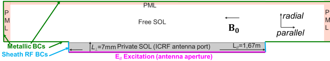
Fig. 1. 2D (radial/parallel) geometry one one SSWICH-SW run (not to scale). The reference dimensions of the idealized antenna port are indicated, as well as the boundary conditions (BCs) enforced at the different boundaries.
