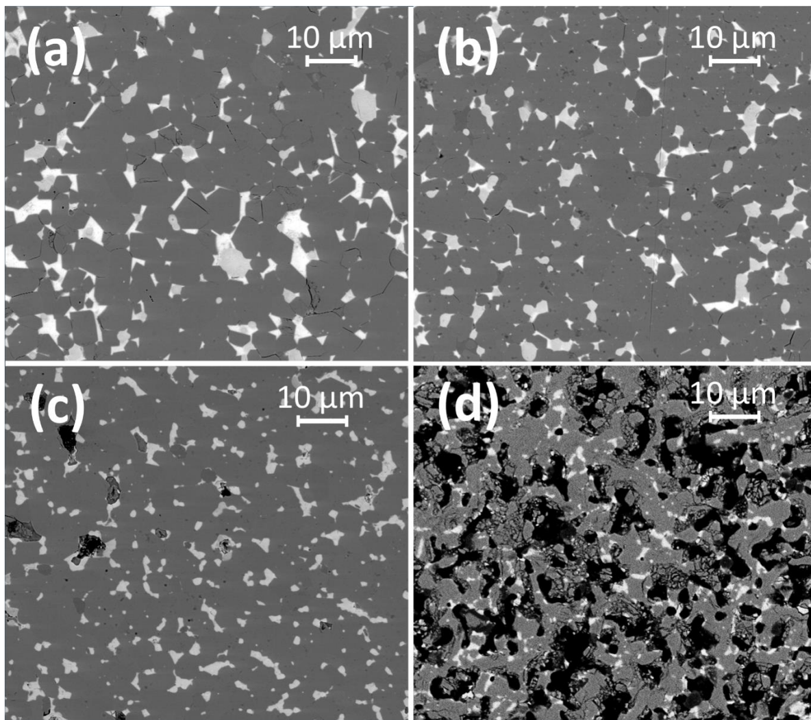
Figure 1-Evolution of the microstructure of a) the conventional processed magnet compared to the PIM produced magnets with b) 1140 ppm of C, c) 5300 ppm of C and d) 8500 ppm of C, observed by SEM-BSE
