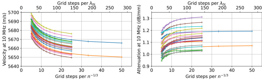
Figure 8: Estimated velocity and attenuation of L waves at 10 MHz as a function of grid resolution for 20 random realizations of steel REVs.
