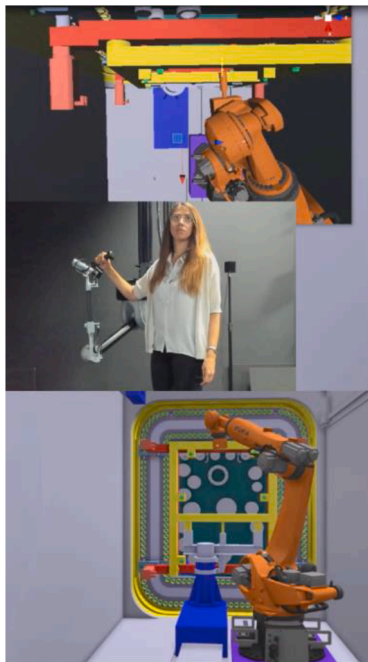
Fig. 14. Accessibility study of the Kuka Robot with force feedback.
