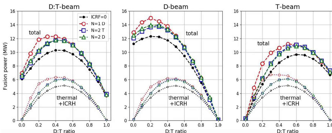
Figure 6. Fusion power estimates as function of the D:T isotope ratio for three NBI injection cases ( P_{NBI}=32\text{MW} , E_{NBI}=120\text{keV} ) and three different ICRF heating schemes ( P_{ICRH} = 4\text{MW} ): Fundamental (N=1) D heating with 1% Be (circles), 2nd harmonic (N=2) T with 0.3% N = 1 ^3\text{He} heating (squares) and N = 2 D with 1% N = 1 H ICRF heating (triangles). The NBI only values (RF = 0) are also shown (small dots). Figure from [55].
