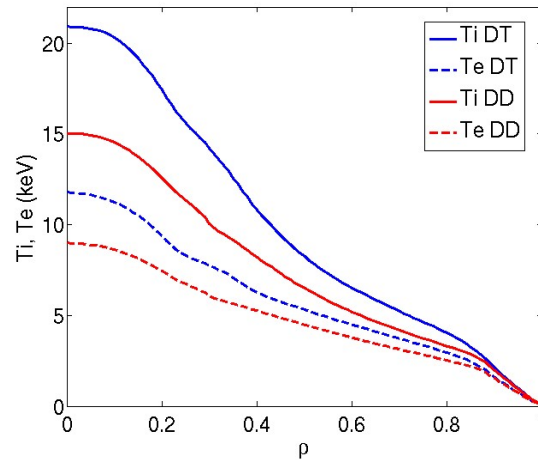
Figure 11. Comparison between Ti and Te for D-T and D in the case of the extrapolated plasmas at input power 40MW from the JET hybrid discharge 86614 with CRONOS and TGLF-SAT0. Figure from [10].
