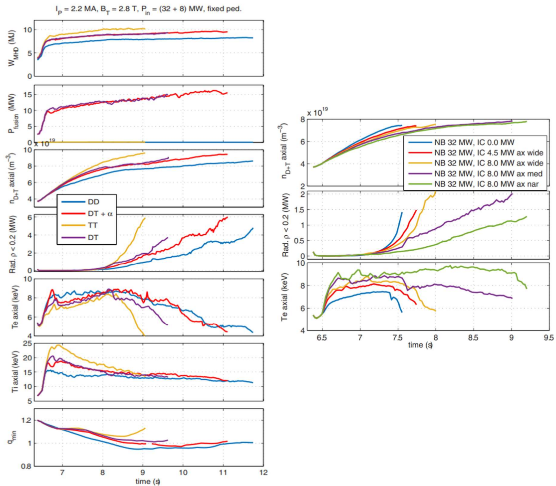
Figure. 10. Predicted time evolution of the total energy ( W_{\text{MHD}} ), fusion power ( P_{\text{fusion}} ), total ion density in the axis ( n_{\text{D+T axial}} ), radiated power inside \rho < 0.2 , Te and Ti at the plasma axis ( T_{\text{e axial}} T_{\text{i axial}} ) and minimum q ( q_{\text{min}} ) (left). Time evolution of n_{\text{D+T axial}} , radiated power inside \rho < 0.2 and Te axial for different assumptions of ICRH power deposition width at the axis: wide, med (medium) and nar (narrow) (right). Figures from [67].
