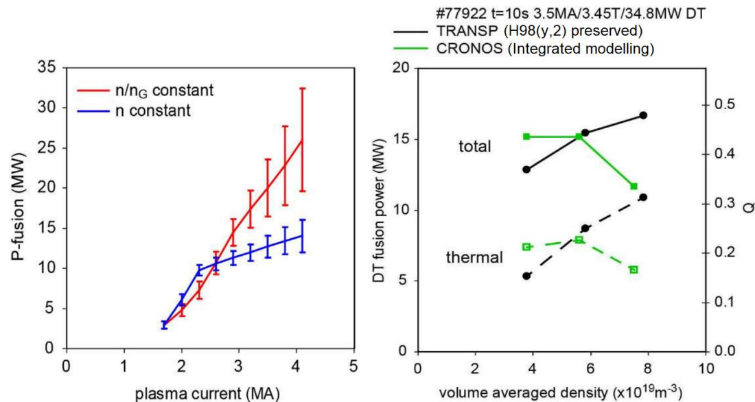
Figure 1. D-T fusion power P_{fus} (P-fusion in left figure) calculated with JETFUZE and the scaling strategy with different assumptions for the density extrapolation. The error bars cover the range due to extrapolations from three conditions from the two reference pulses, #75225 at t=6.5s and t=8s and #77922 at t=10s . Figure from [7] (left). Comparison between P_{fus} and Q calculated with TRANSP from an extrapolation of the discharge #77922 preserving H_{98}(y,2) and with the fully predictive simulation using CRONOS and BGB model for heat transport as a function of volume-averaged density (right).
