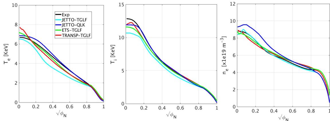
Figure 9. Comparison between the experimental and simulated T_e , T_i and n_e with TGLF-SAT1 and QLK for the discharge #97781. Figure from [51].
