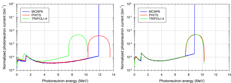
Fig. 3. Normalized energy spectra of photon neutrons emitted by the deuterium target irradiated by 20 MeV photons, simulated with MCNP6, PHITS and TRIPOLI-4. On the left, with ENDF/B-VIII.0. On the right, with JENDL-5.
