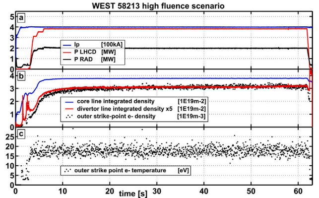
Fig. 2. Time traces of a representative plasma pulse from the High fluence campaign of 2023, lasting about 60 s. (a) Plasma current (blue), lower hybrid power coupled to the plasma (red), and total radiated power (black). (b) Time traces of core line integrated density (blue), divertor line integrated density \times 5 (red) from interferometry, and outer strike point electron density measured by Langmuir probe (black dots). (c) Outer strike point electron temperature from Langmuir probe. (For interpretation of the references to color in this figure legend, the reader is referred to the web version of this article.)
