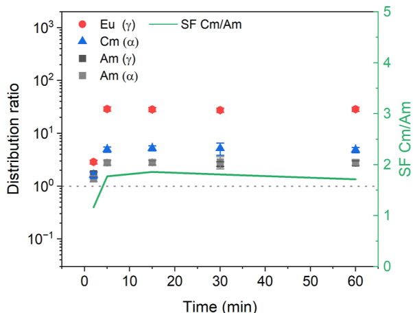
Figure 3. Distribution ratios as a function of mixing time with iPDdDGA. Aq: 10^{-3}\text{ mol}\cdot\text{L}^{-1} Ln + 3\text{ kBq/mL} ^{152}\text{Eu} , ^{241}\text{Am} , and ^{244}\text{Cm} radiotracers in 3\text{ mol}\cdot\text{L}^{-1} \text{HNO}_3 . Org: 0.005\text{ mol}\cdot\text{L}^{-1} iPDdDGA dissolved in 10\%_{\text{Vol}} 1-octanol in n -dodecane, 2\times pre-equilibrated with 3\text{ mol}\cdot\text{L}^{-1} \text{HNO}_3 . A/O: 1, 1900 rpm, 20\text{ }^\circ\text{C} .
