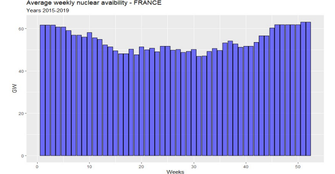
French nuclear fleet's average availability - 63 GWe (2015-2019)
