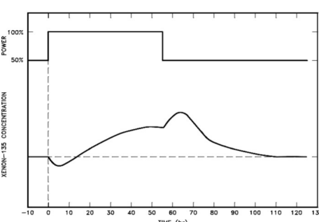
Xenon 135 variations during power changes, U.S. Department of Energy (1993)
