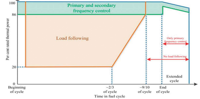
Minimal power limits during a fuel cycle in a French PWR, IAEA (2018)
