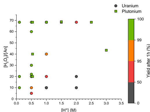
Figure 1 : Precipitation yield of pure uranium and plutonium peroxide depending on the initial acidity and molar ratio between actinide and hydrogen peroxide ; [U(VI)]_{ini} = [Pu(IV)]_{ini} = 0.068 M
