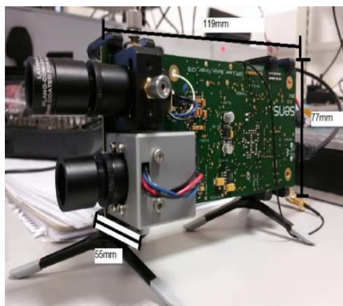
Figure 7. Long-range LiDAR prototype brought to the project.
