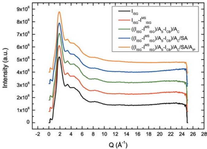
Figure 6 Corrections applied to the ISG intensity integrated pattern. From bottom to top: intensities related to ISG glass, ISG glass - MS, [(ISG glass MS)/ A_S - CB]/ A_C , [(ISG glass MS)/ A_S - CB]/ A_C /SA and [(ISG glass MS)/ A_S - CB]/ A_C /SA/ A_{IP} [see equation (1) for details]. Polarization and geometric g corrections are taken into account during the FIT2D integration procedure. The curves are displaced vertically for clarity.
