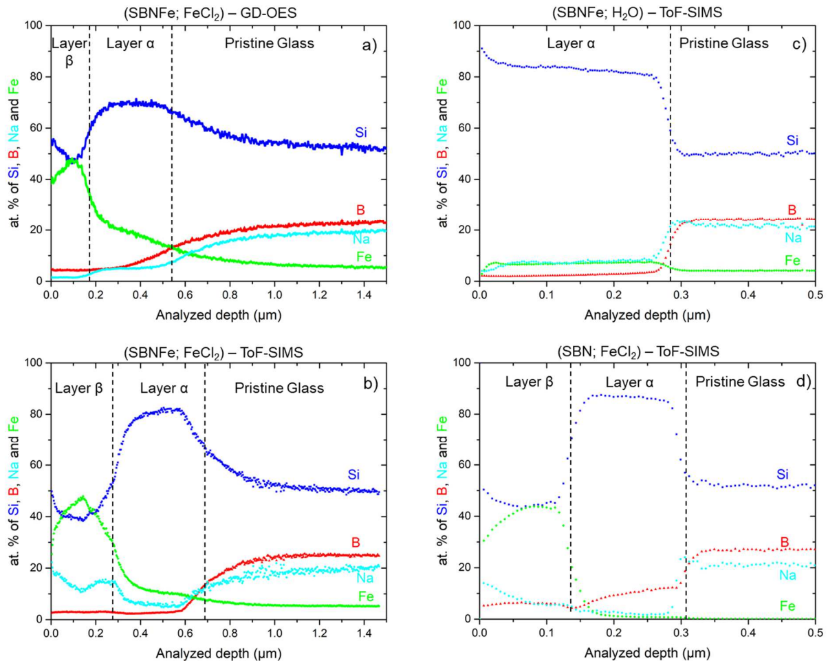
440 Figure 5. Si, B, Na and Fe depth profiles (in at.% normalized with respect to the sum of Si, B, Na and Fe contents) recorded on monoliths altered at 50°C and free pH during 323 days ( S/V = 20\,000\text{ m}^{-1} ). a) GD-OES profiles recorded on sample from (SBNFe; FeCl 2 ) experiment. b-d) ToF-SIMS profiles recorded on samples from (SBNFe; FeCl 2 ), (SBNFe; H 2 O) and (SBN; FeCl 2 ) experiments, respectively. Black dotted lines delineate the interfaces between successive layers.
