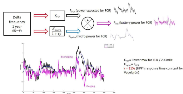
Figure 3: Power extraction methodology
