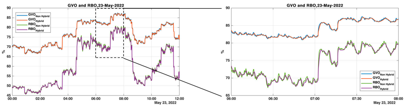
Figure 21. Comparison of the simulated guide vane opening and runner blade opening in hybrid and non-hybrid mode.
