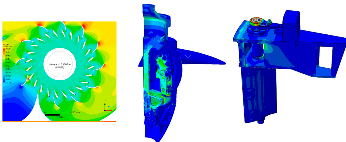
Figure 8. Flow condition at the guide vanes (left); Stress amplitude results at runner and guide vane mechanism finite element model (middle and right).
