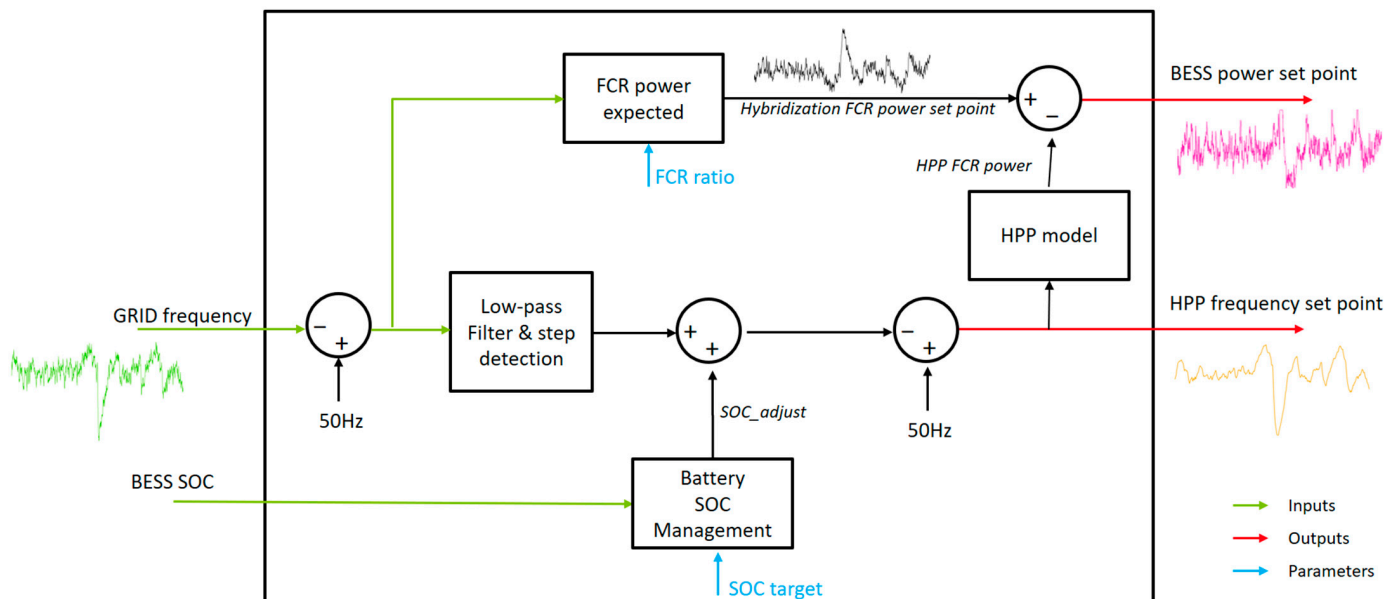
Figure 3. Control algorithm overview.
