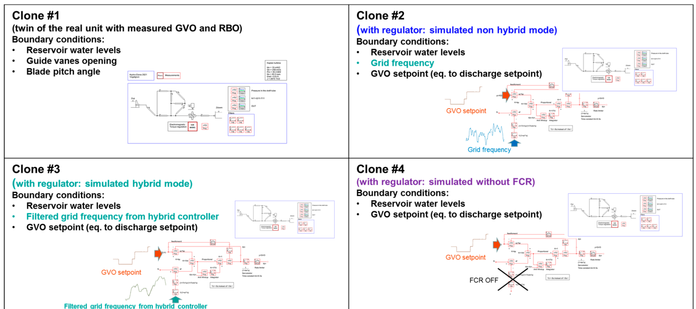
Figure 15. Summary and characteristics of the four real-time models deployed in Hydro-Clone.
