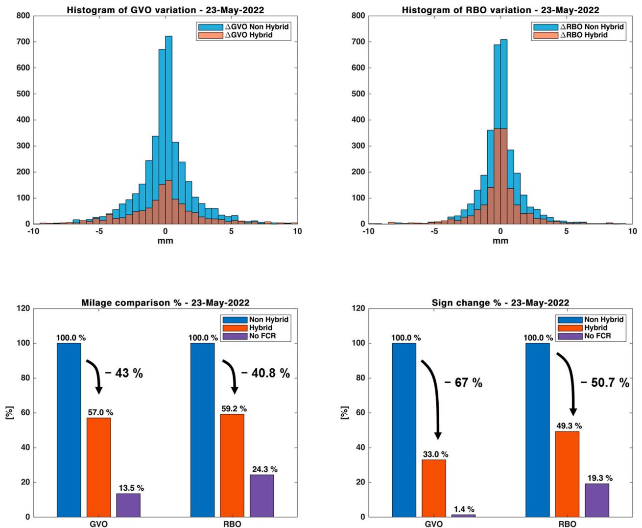
Figure 22. Assessment of the reduction in mileage and number of sign changes for the guide vane opening (GVO), and runner blade opening (RBO), in hybrid mode.
