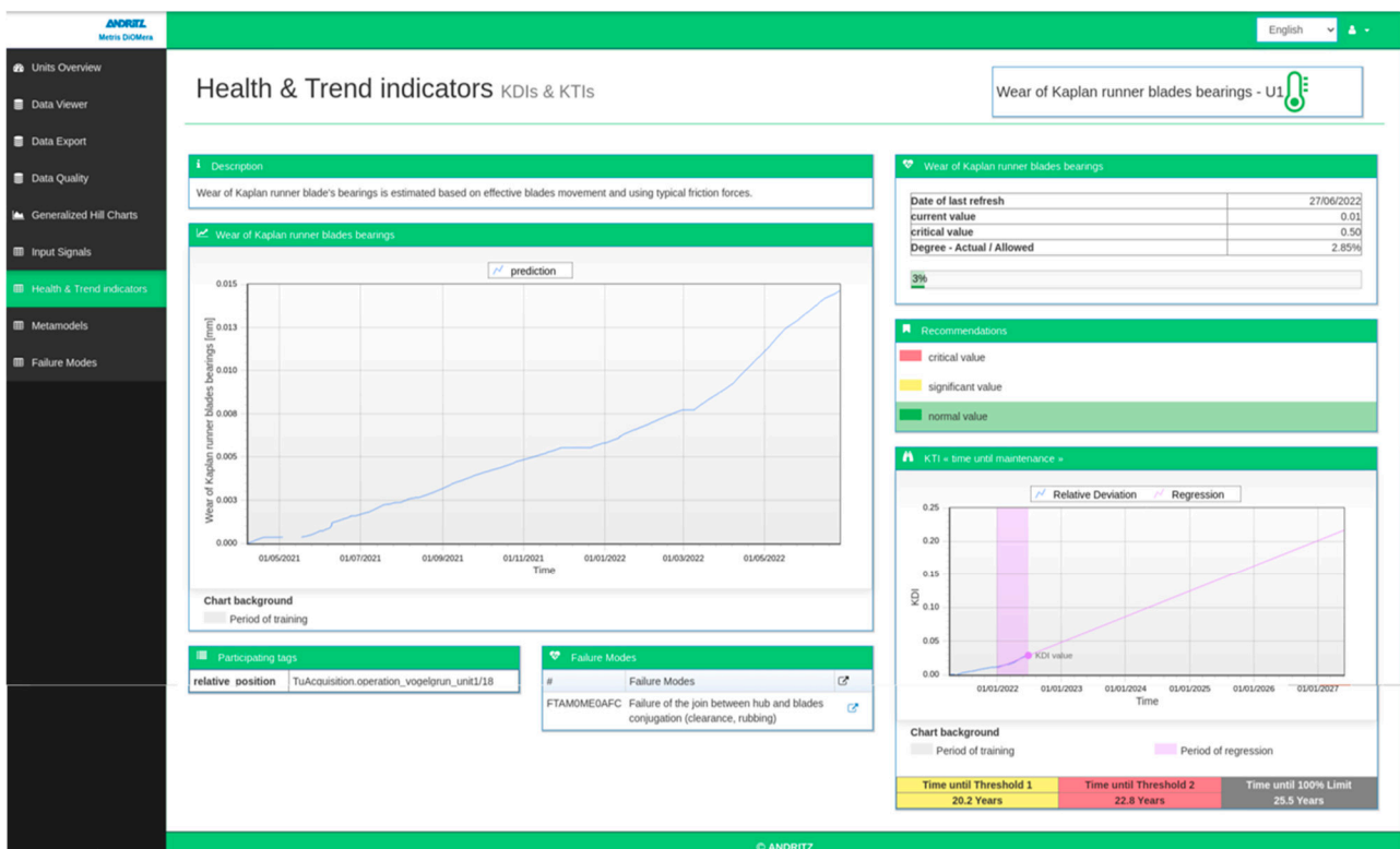
Figure 20. Metris DiOMera page summarizing the wear of runner blade bearing indicator of unit 1.
