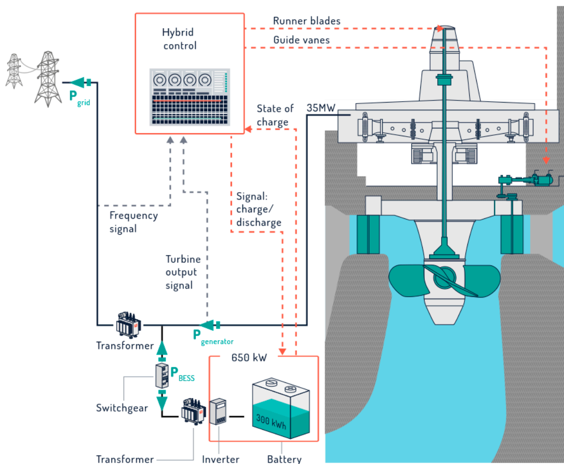
Figure 2. Overview of the hybrid unit setup.
