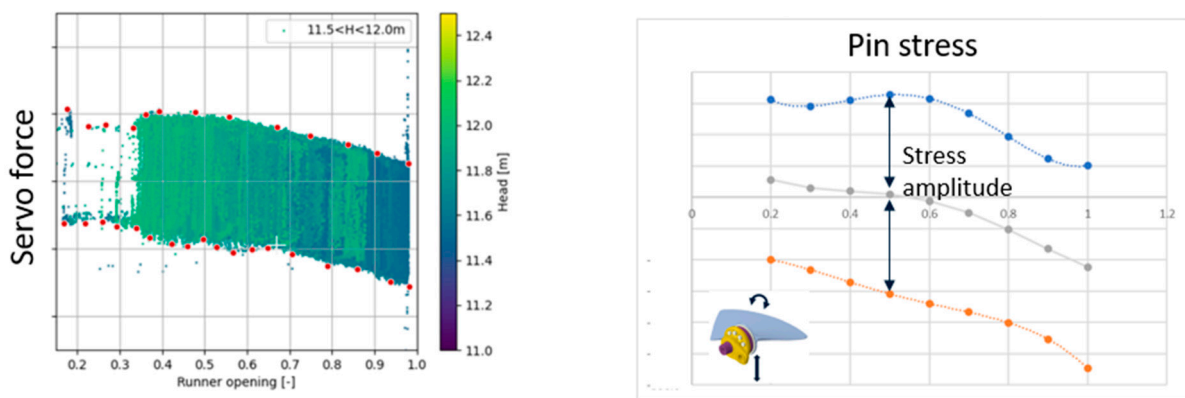
Figure 19. Measured servomotor forces and related pin stress.
