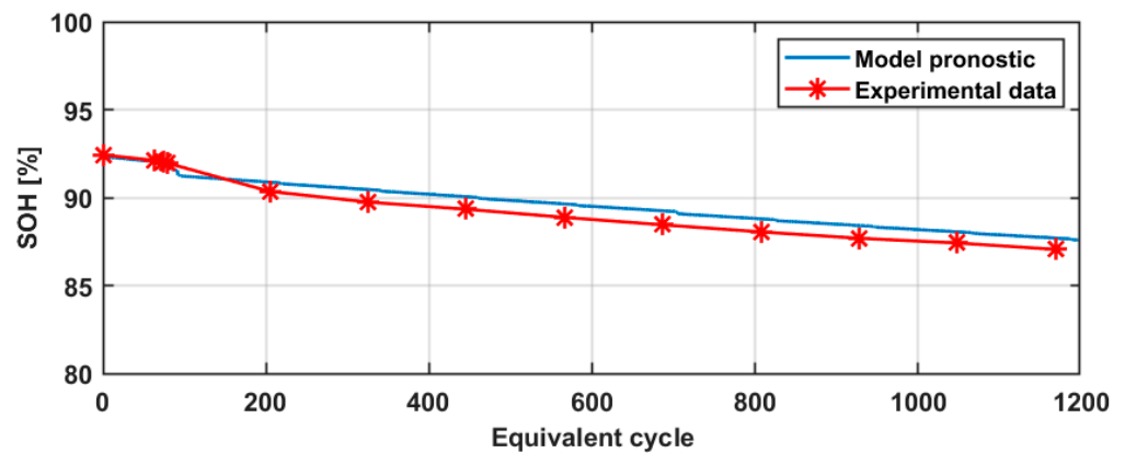
Figure 6. Experimental results vs. model prognostic comparison.
