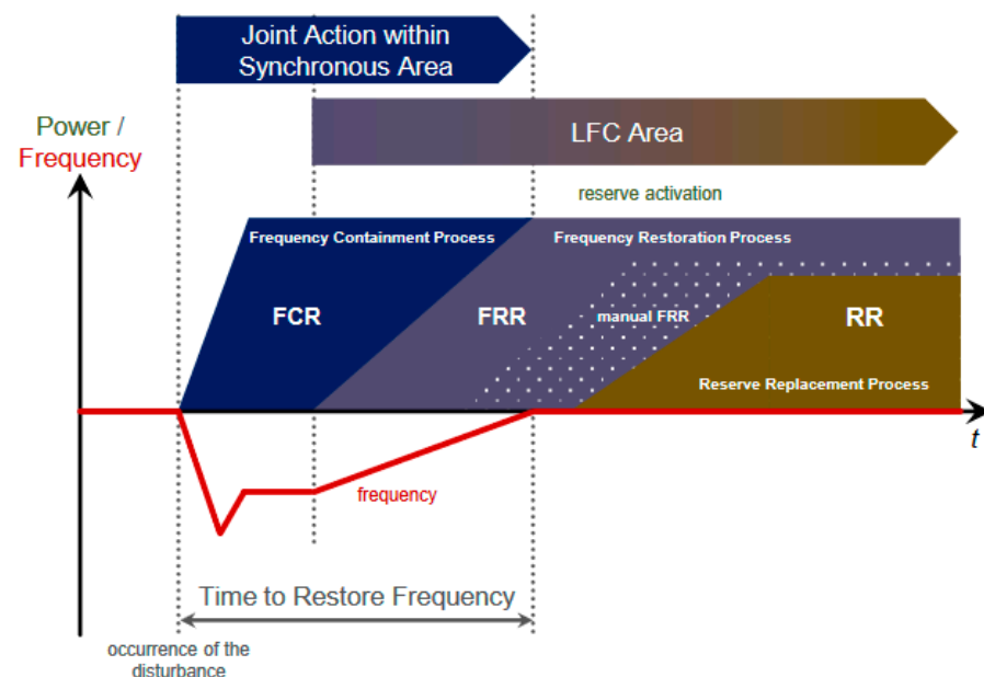
Figure 1. Dynamic hierarchy of load-frequency control processes [7].
