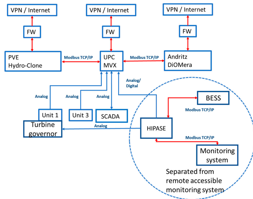
Figure 7. Overview of monitoring concept.
