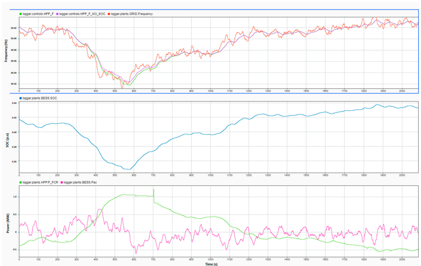
Figure 5. Simulation of BESS operation with SoC management implementation.
