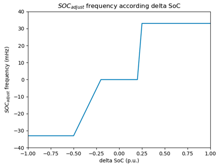
Figure 4. Frequency adjustment algorithm.
