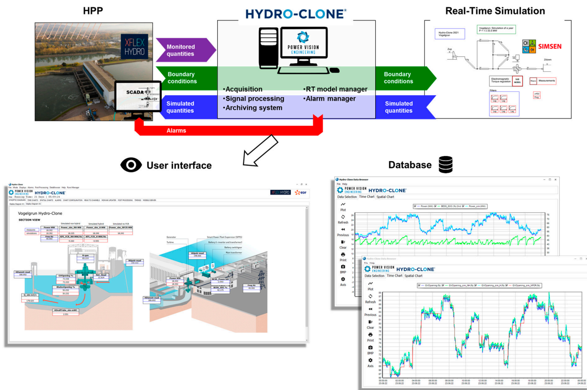
Figure 14. General concept of Hydro-Clone system based on real-time simulation.
