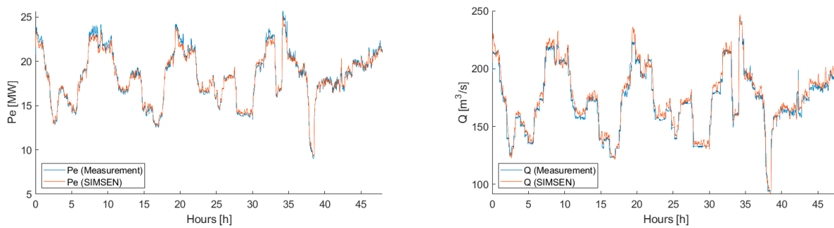
Figure 13. Comparison of power and discharge measurements (blue line) made over 2 days in April 2021 and numerical results (red line).
