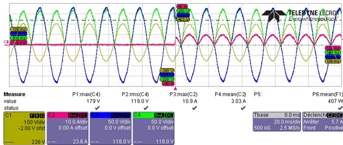
Figure 13. Start of SRB charging with electrical grid.
