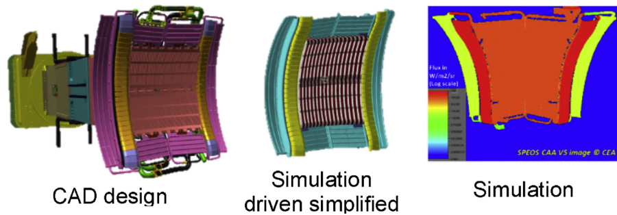
Fig. 2. LHC antenna photonic simulation with SPEOS.
