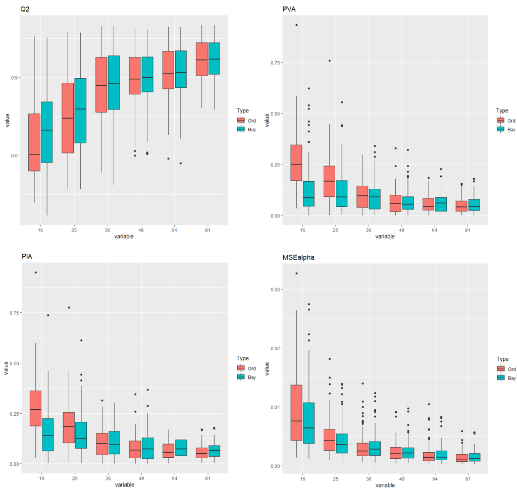
Figure 2 - Validation criterion against data size for simulated data for Q^2 criterion, PVA criterion, PIA criterion and MSE\alpha criterion.
