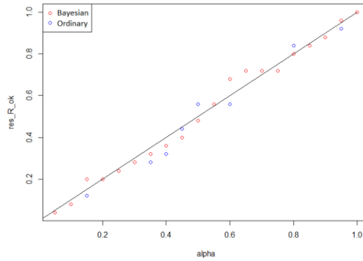
Figure 1 Example of an \alpha -CI plot with both Bayesian and ordinary kriging
