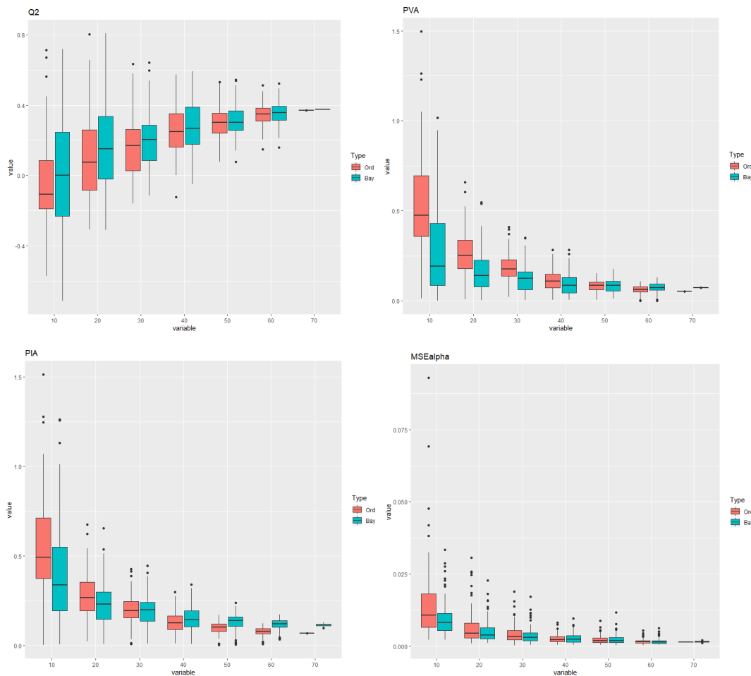
Figure 3 - Validation criterion against data size for the G3 data set for Q^2 criterion, PVA criterion, PIA criterion and MSE\alpha criterion.
