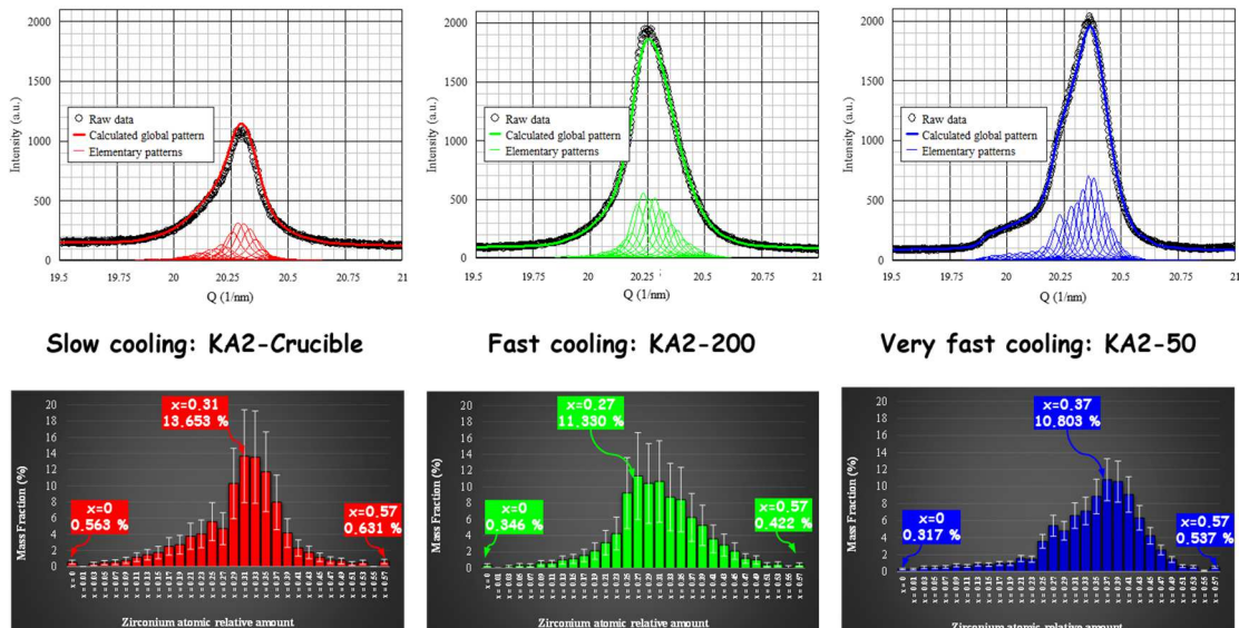
Fig. 4. Cationic composition fluctuations into corium crystals as a function of the cooling process.
