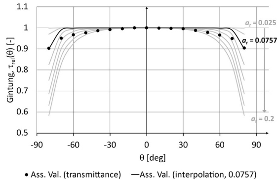
Figure 5: Assigned values for the relative angular transmittance measurements of Gintung (black dots), compared with the assigned values for the interpolation with a_r = 0.0757 (black line), and a set of interpolations from a_r = 0.025 to a_r = 0.2 (step 0.025, grey lines).
