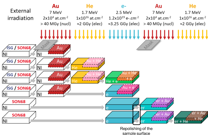
Figure 1: Scheme of the irradiation scenarios performed on the glass coupons.
