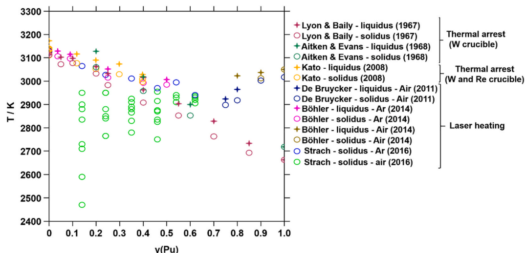
Fig. 1. Experimental melting data available in the literature for U_{1-y}Pu_yO_2 .
