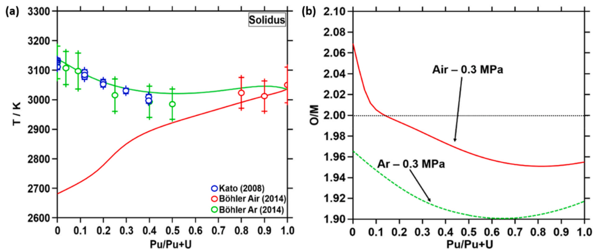
Fig. 14. Calculated (a) solidus temperatures compared to the experimental data of Kato et al. [19] and Böhler et al. [5] and (b) O/M ratio at the solidus temperature as a function of Pu content, under air in red and argon in green. The calculations were performed for 5 mol of gas and 3 mol of samples.
