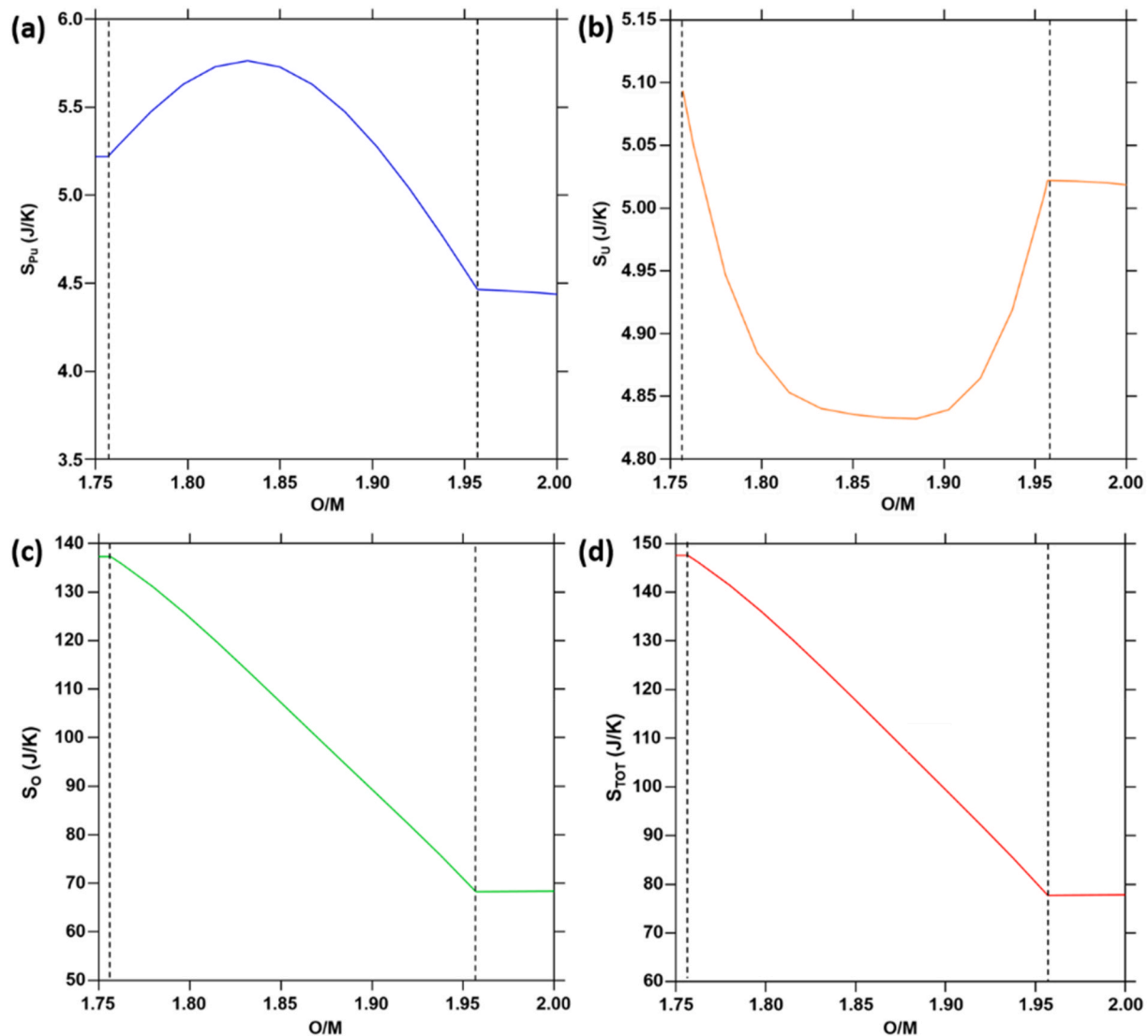
Fig. 12. Configurational entropy of (a) Pu, (b) U, (c) O and (d) total at 3000 K as a function of the O/M ratio for y = 0.50 .
