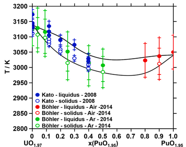
Fig. 5. UO 1.97 –PuO 1.95 phase diagram compared with the selected experimental data of Kato et al. [19] and Böhler et al. [5].
