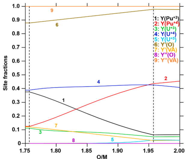
Fig. 13. Calculated site fractions at 3000 K as a function of the O/M ratio for y = 0.50 .
