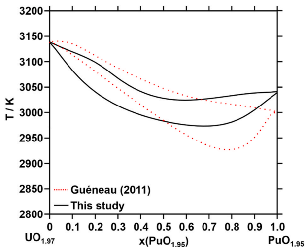
Fig. 4. Calculated UO 1.97 –PuO 1.95 phase diagram compared to Guéneau et al. (dashed line) [7].
