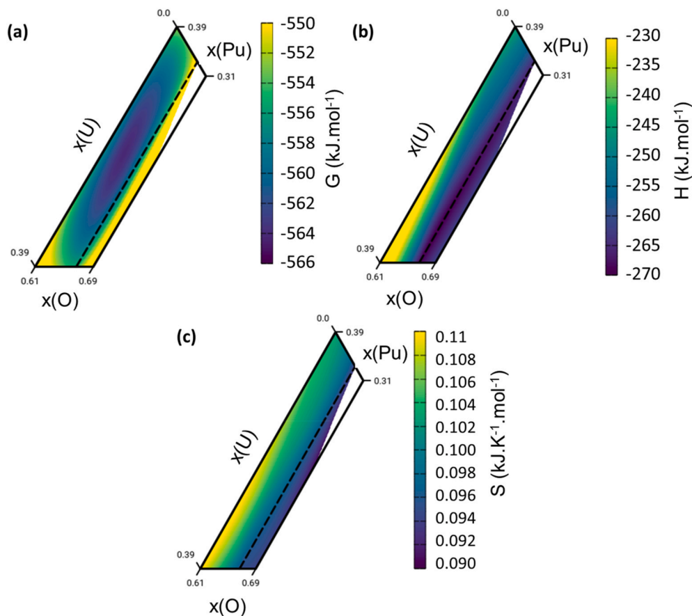
Fig. 11. Maps of (a) the Gibbs energy, (b) the enthalpy, (c) the entropy of U_{1-y}Pu_yO_{2\pm x} mixed oxide as a function of the composition in mole fraction at 3000 K.
