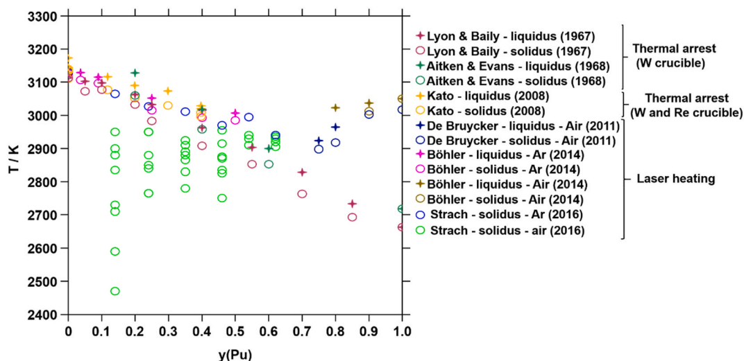
Fig. 1. Experimental melting data available in the literature for U_{1-y}Pu_yO_2 .
