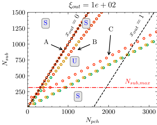
(b) Marginal stability lines in the EXOCET configuration based on the criterion of [17].
