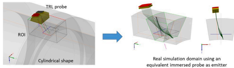
Fig. 17. 3D weld configuration with a TRL probe and the simulated Region Of Interest (ROI).
